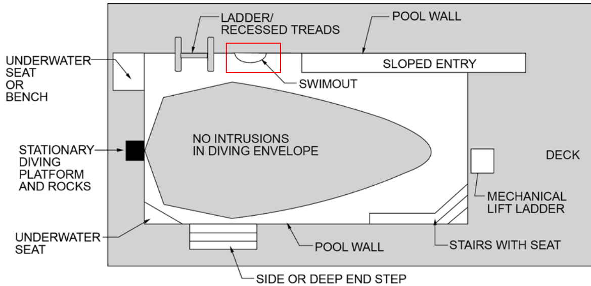
FIGURE 322.2 MINIMUM DIVING WATER ENVELOPE
