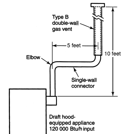
FIGURE G 101.3 SINGLE DRAFT HOOD-EQUIPPED APPLIANCE – EXAMPLE 1
