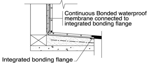
Configuration of base with integrated bonding flange
