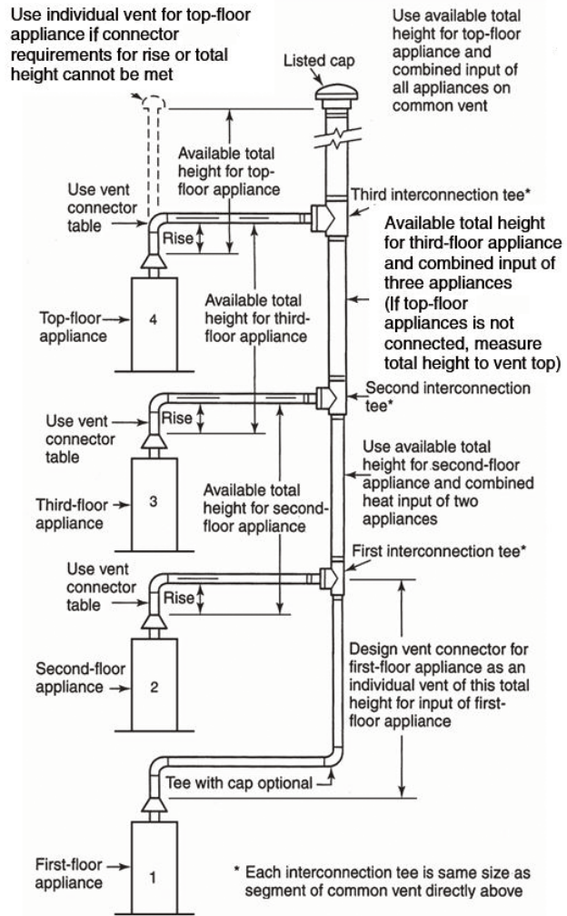
FIGURE G 101.2(14) PRINCIPLES OF DESIGN OF MULTISTORY VENTS USING VENT CONNECTOR AND COMMON VENT DESIGN TABLES
