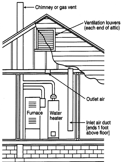
FIGURE 506.4.1(2) ALL COMBUSTION AIR FROM OUTDOORS THROUGH VENTILATED ATTIC [NFPA 54: FIGURE A.9.3.3.1(1)(b)]
