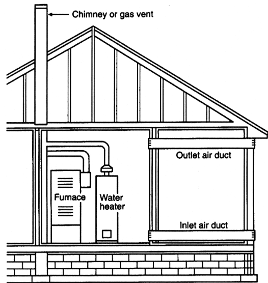
FIGURE 506.4.1(3) ALL COMBUSTION AIR FROM OUTDOORS THROUGH HORIZONTAL DUCTS [NFPA 54: FIGURE A.9.3.3.1(2)]
