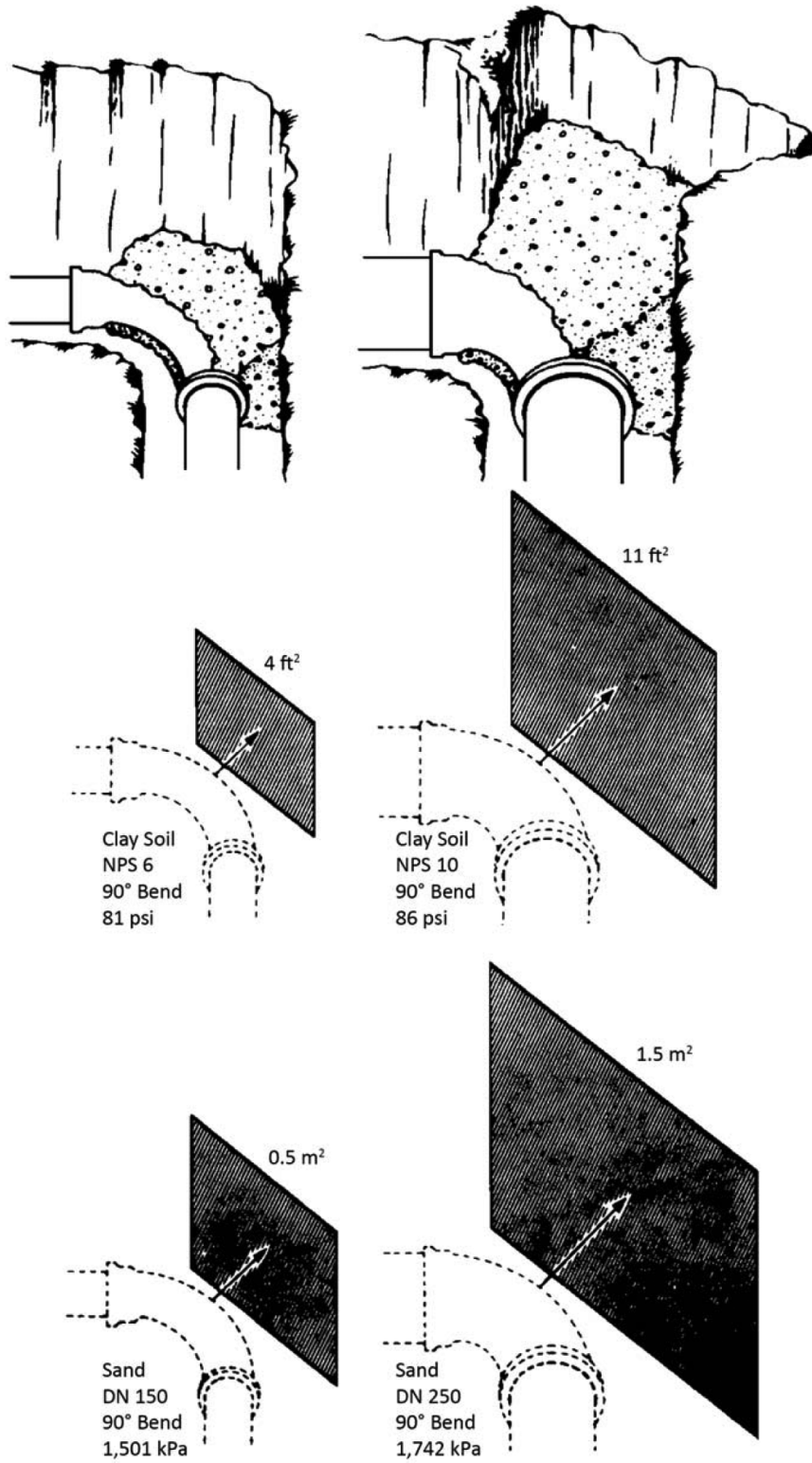
FIGURE 2 THRUST BLOCK BEARING AREA (See Section 5.2.2)
