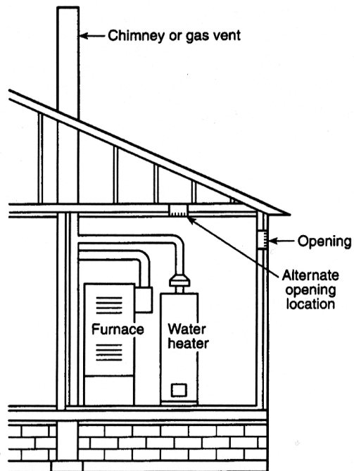
FIGURE 506.4.2 ALL COMBUSTION AIR FROM OUTDOORS THROUGH SINGLE COMBUSTION AIR OPENING [NFPA 54: FIGURE A.9.3.3.2]
