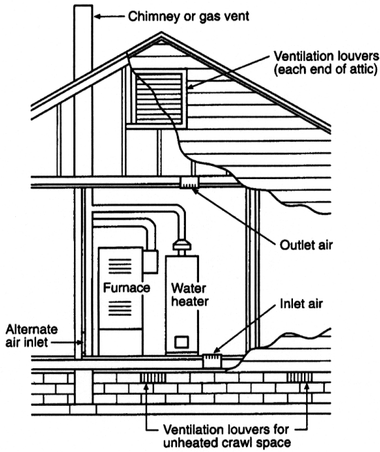
FIGURE 506.4.1(1) ALL COMBUSTION AIR FROM OUTDOORS – INLET AIR FROM VENTILATED CRAWL SPACE AND OUTLET AIR TO VENTILATED ATTIC [NFPA 54: FIGURE A.9.3.3.1(1)(a)]
