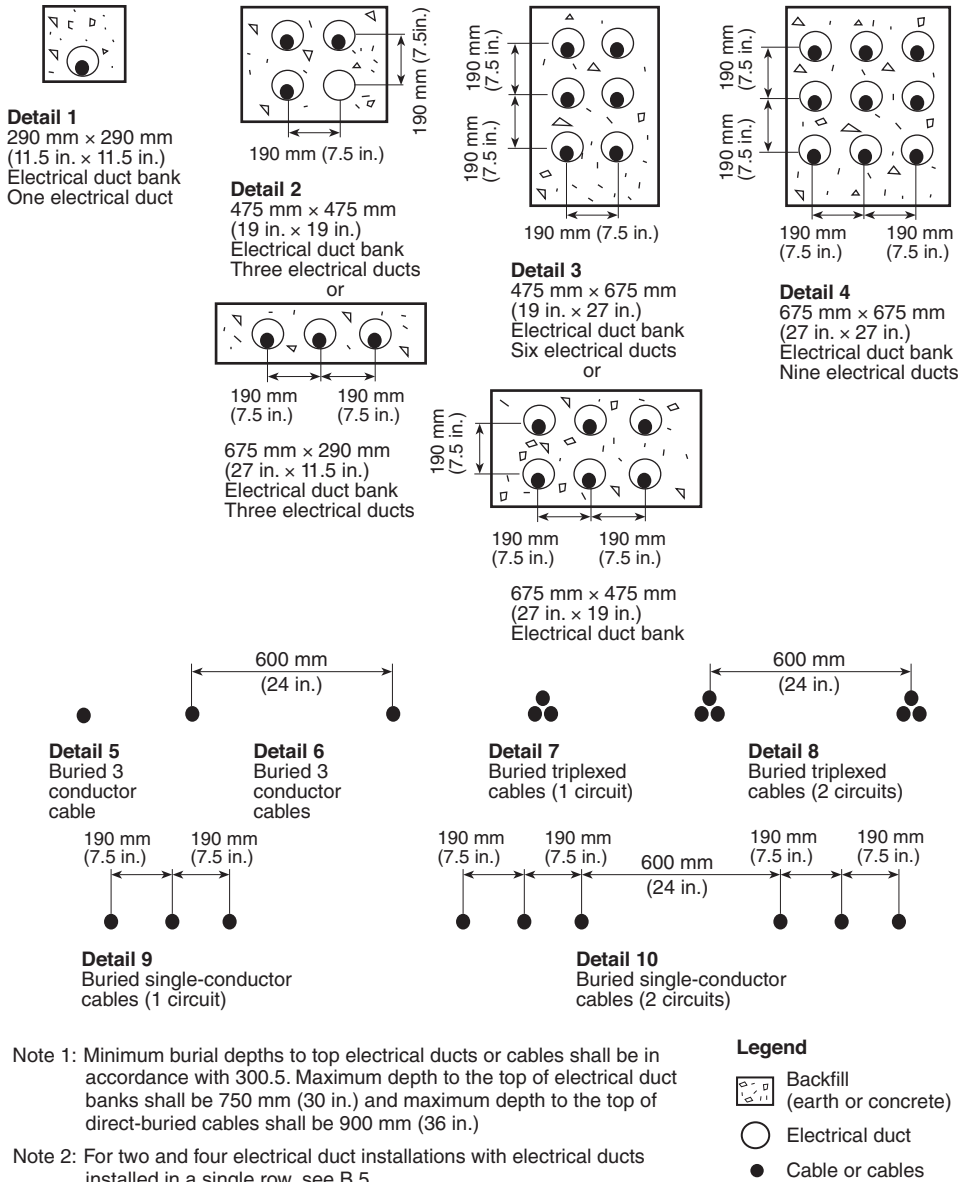
△ FIGURE B.2(1) Cable Installation Dimensions for Use with Table B.2(5) Through Table B.2(10).
