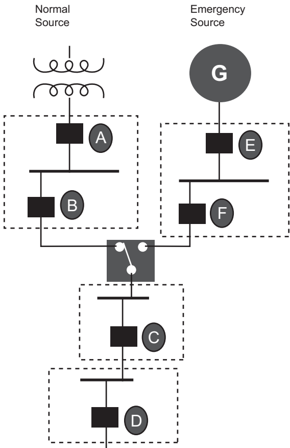
N Informational Note Figure 701.32 Legally Required Standby System Selective Coordination.
