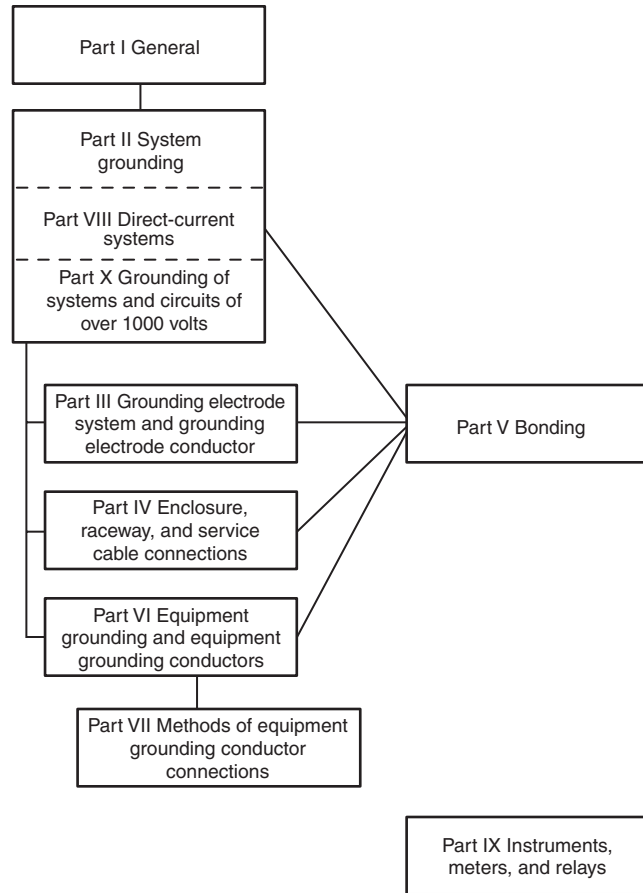
Δ FIGURE 250.1 Grounding and Bonding.
