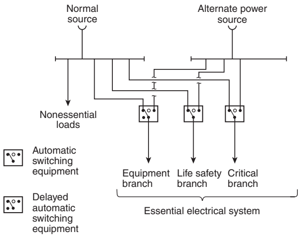
Δ Informational Note Figure 517.31(a) Type 1 Essential Electrical System — Minimum Requirement (greater than 150 kVA) for Transfer Switch Arrangement.
