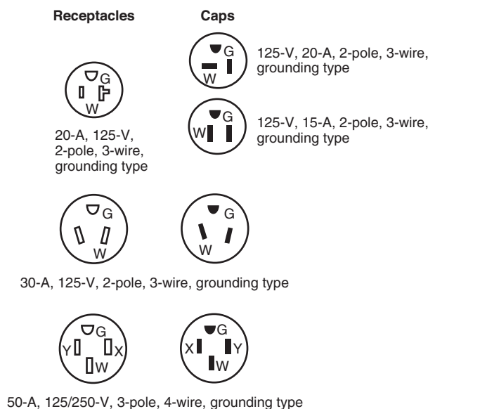
FIGURE 551.46(C)(1) Configurations for Grounding-Type Receptacles and Attachment Plug Caps Used for Recreational Vehicle Supply Cords and Recreational Vehicle Lots.
