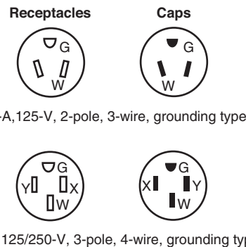
FIGURE 552.44(C)(1) Attachment Cap and Receptacle Configurations.
