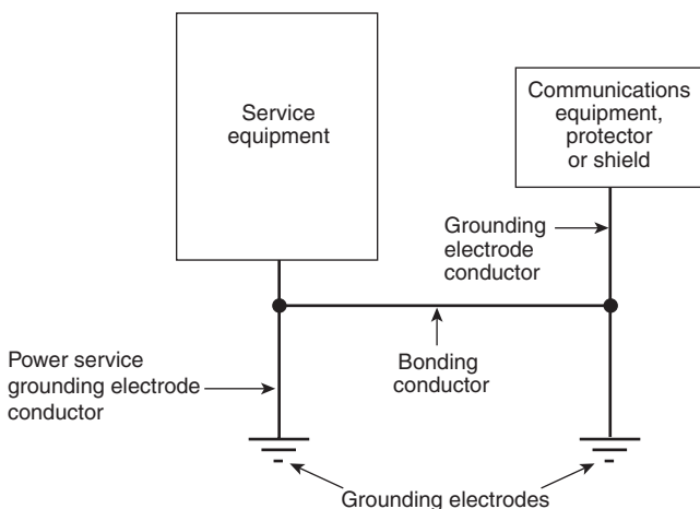
N Informational Note Figure 800.100(B)(2) Illustration of a Bonding Conductor in a Communications Installation.
