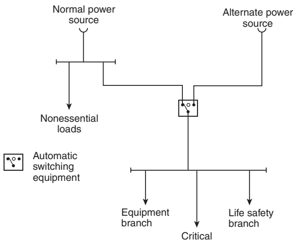
Δ Informational Note Figure 517.31(b) Type 1 Essential Electrical System — Minimum Requirement (150 kVA or less) for Transfer Switch Arrangement.
