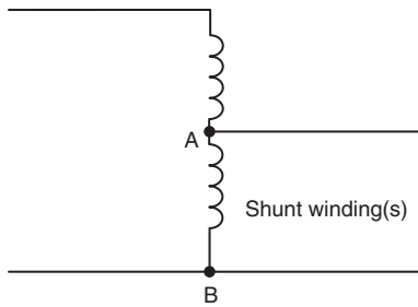
FIGURE 450.4(A) Autotransformer.
