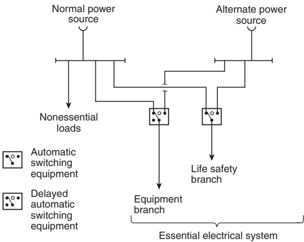
Informational Note Figure 517.42(a) Type 2 Essential Electrical Systems (Nursing Home and Limited Health Care Facilities) — Minimum Requirement (greater than 150 kVA) for Transfer Switch Arrangement.
