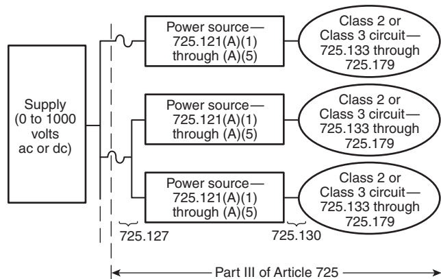
Δ Informational Note Figure 725.121 Class 2 and Class 3 Circuits.
