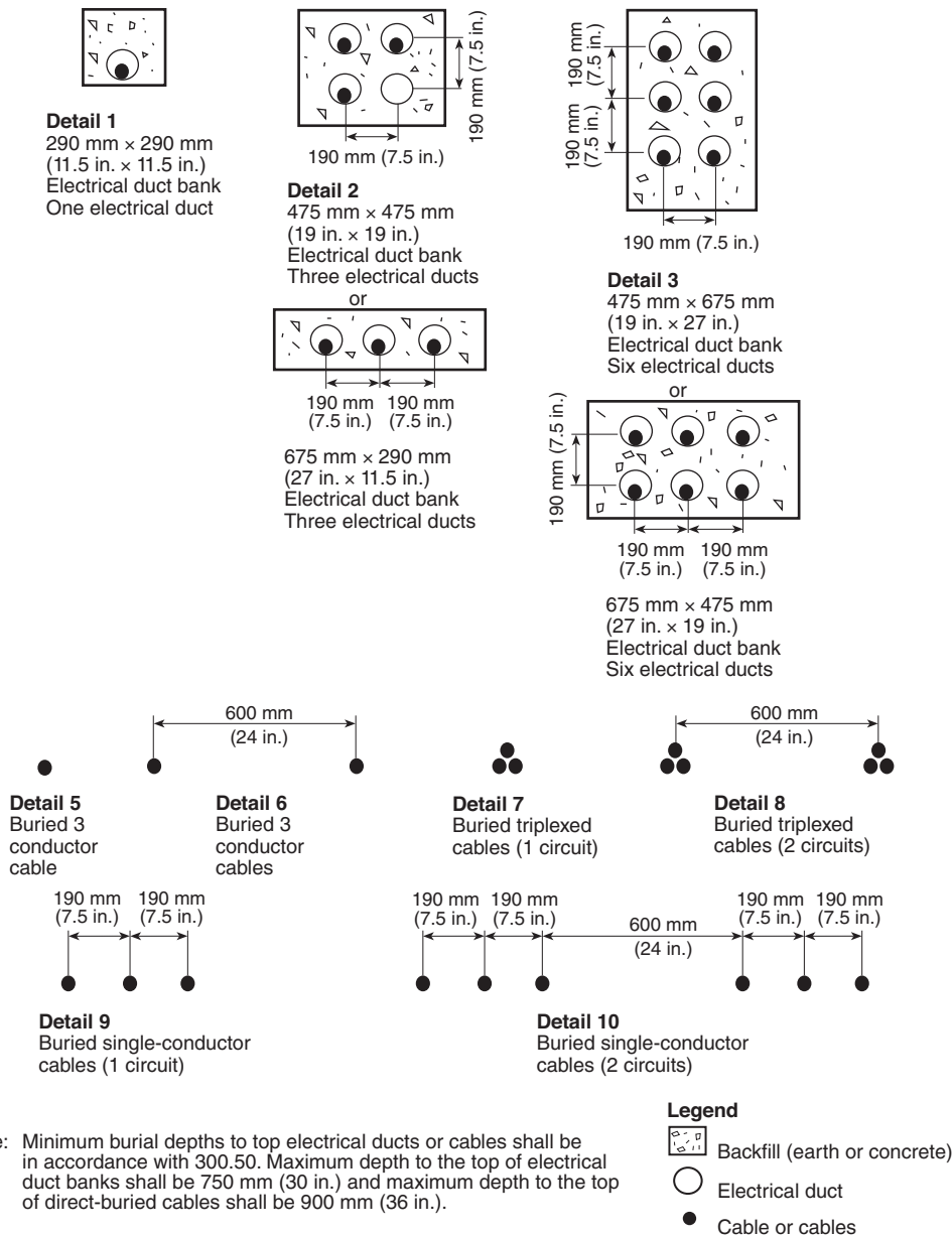
▲ FIGURE 311.60(D)(3) Cable Installation Dimensions for Use with Table 311.60(C)(77) Through Table 311.60(C)(86).
