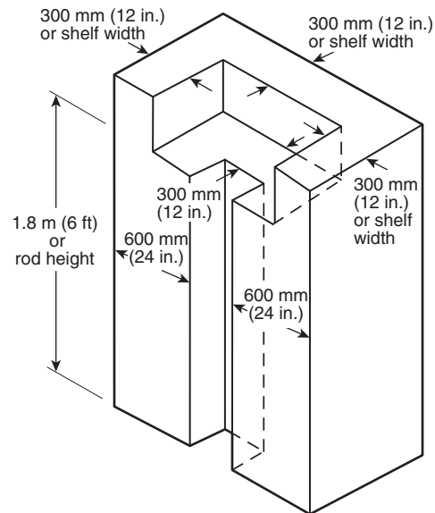
FIGURE 410.2 Clothes Closet Storage Space.
