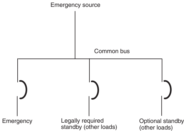
Δ Informational Note Figure 700.10(B)(a) Single or Multiple Feeders Without Overcurrent Protection.
