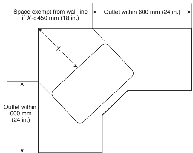
Range, counter-mounted cooking unit, or sink mounted in corner
