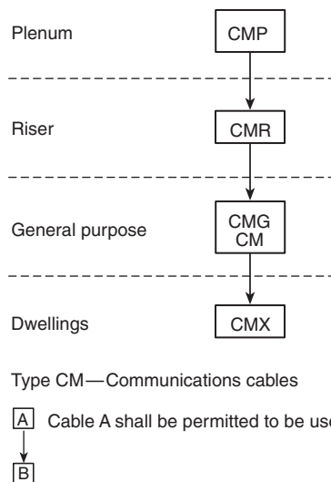
FIGURE 805.154 Cable Substitution Hierarchy.
