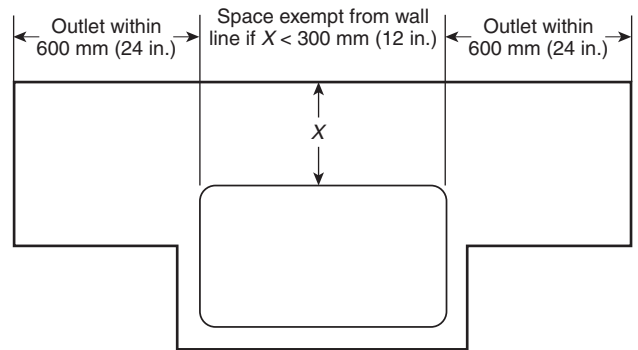
Range, counter-mounted cooking unit, or sink extending from face of counter
