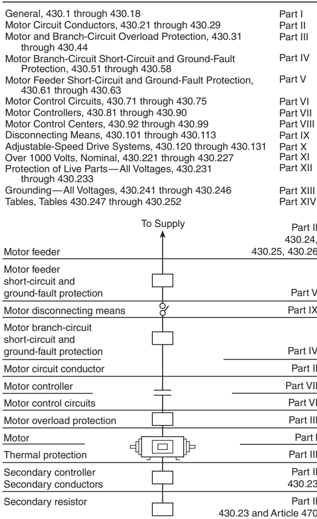
▲ FIGURE 430.1 Article 430 Contents.
