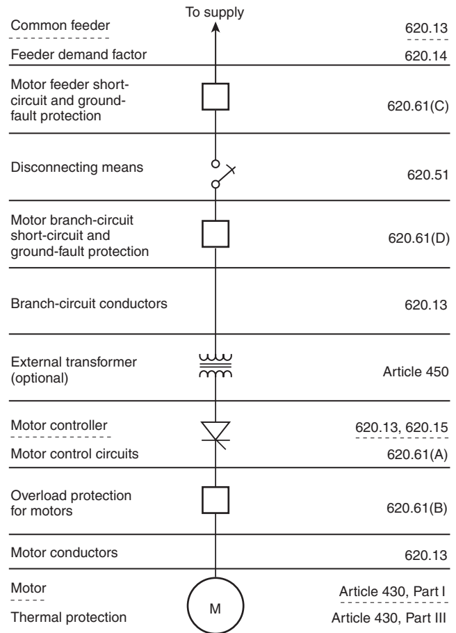
Informational Note Figure 620.13 Single-Line Diagram.
