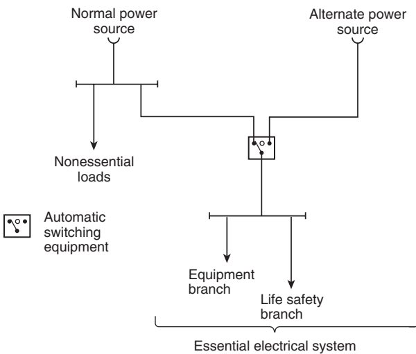
Informational Note Figure 517.42(b) Type 2 Essential Electrical Systems (Nursing Home and Limited Health Care Facilities) — Minimum Requirement (150 kVA or less) for Transfer Switch Arrangement.
