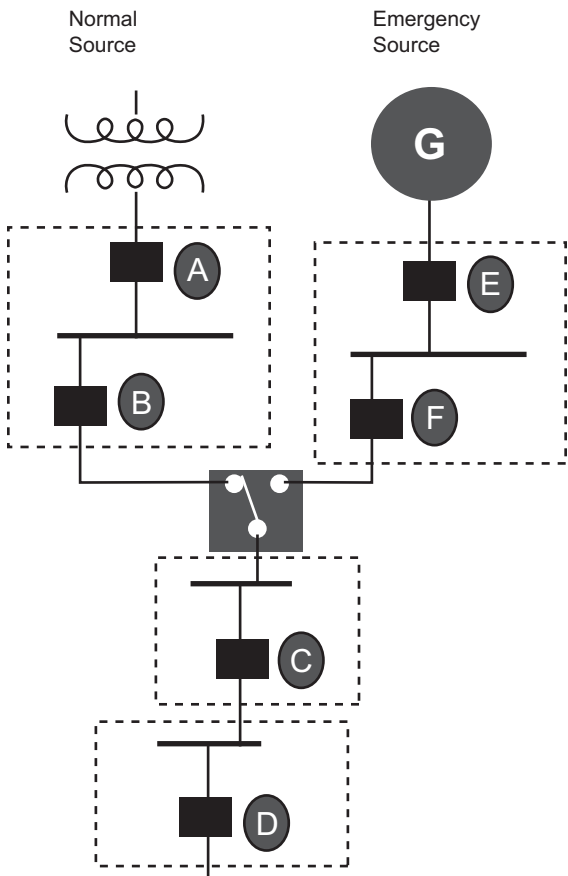
Informational Note Figure 708.54 Critical Operations Power System Selective Coordination.
