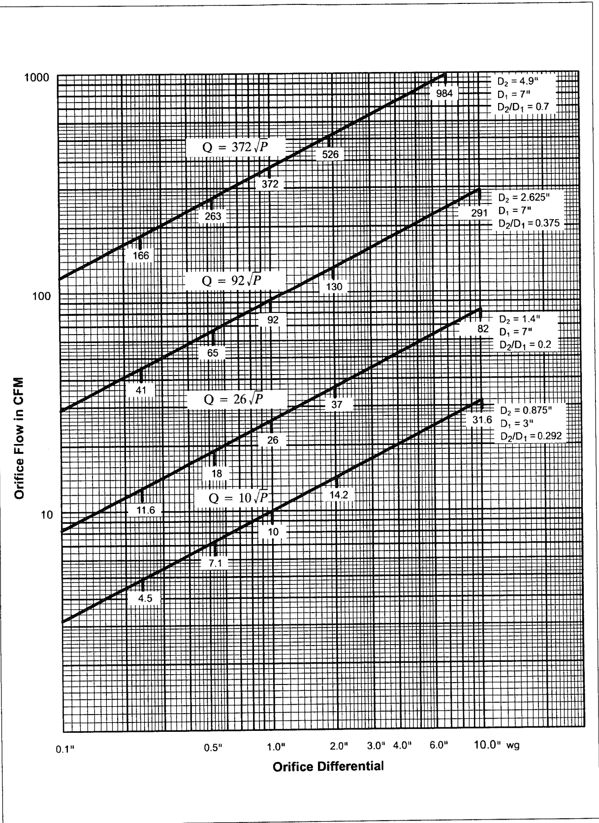
FIGURE 5-3 TYPICAL ORIFICE FLOW CURVES
