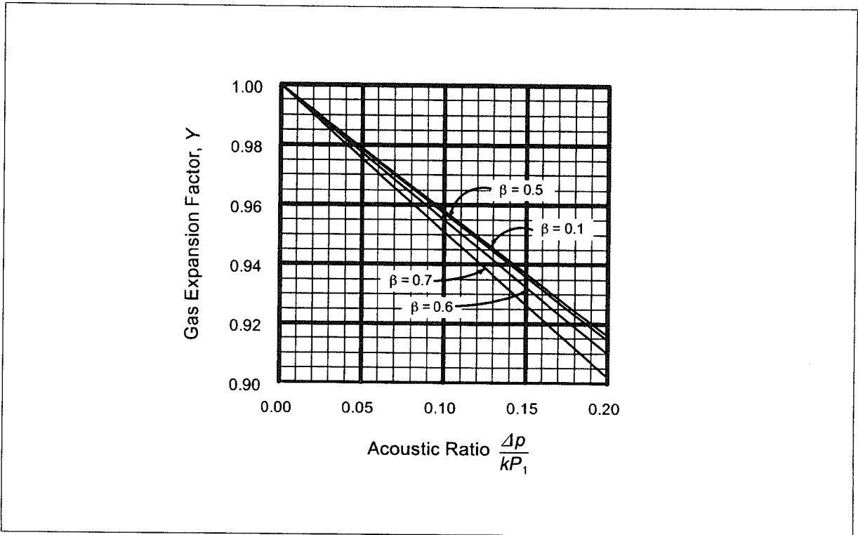
FIGURE L-1 GAS EXPANSION FACTOR, Y, VERSUS ACOUSTIC RATIO, \Delta P/KP_1
