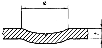
Figure A.2 — Dent containing cut or gouge
