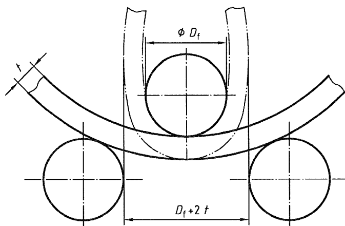
Figure 8 — Illustration of bend test
