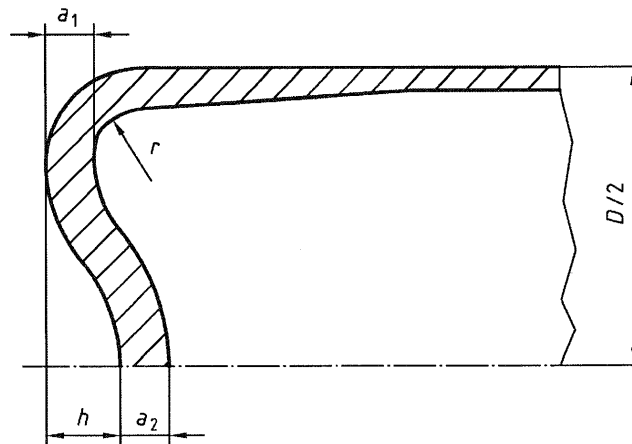
Figure 2 — Concave base ends
