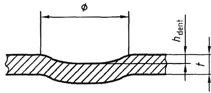
Figure A.1 — Dent
