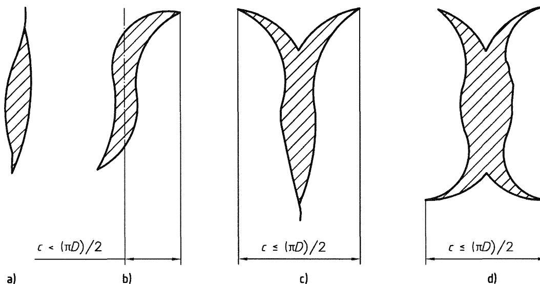
Figure 5 — Acceptable burst profiles
