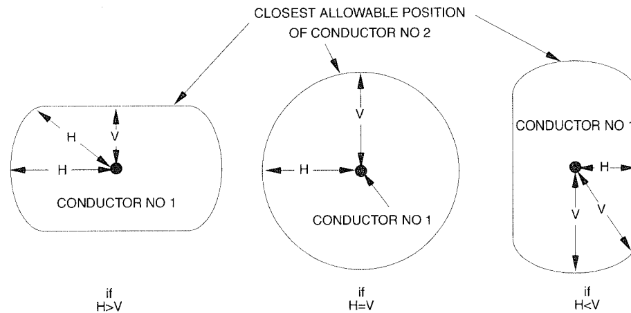
Figure 233-3—Clearance envelope
