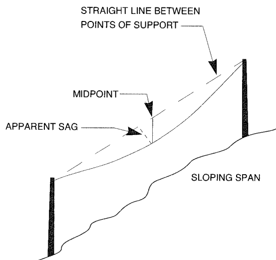
Figure D-1—Sag and apparent sag
