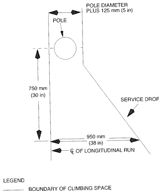
Figure 236-1—Rule 236G, Exception 3
