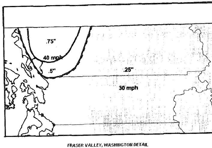
Figure 250-3(d)—Uniform ice thickness with concurrent wind
