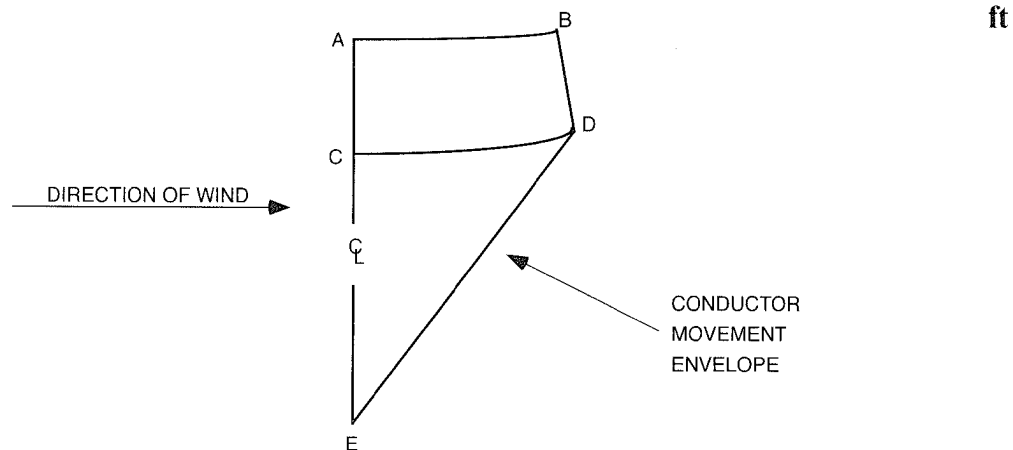
Figure 233-2—Conductor movement envelope
