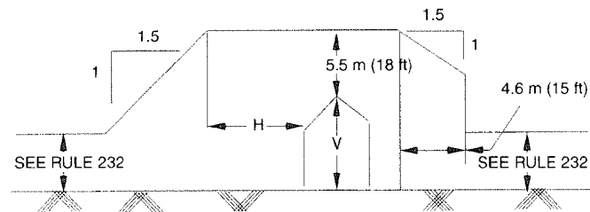
Figure 234-4(a)—Clearance envelope for grain bins filled by permanently installed augers, conveyors, or elevators
