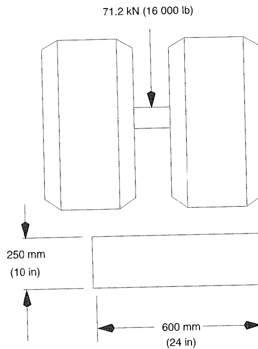
Figure 323-2—Wheel load area
