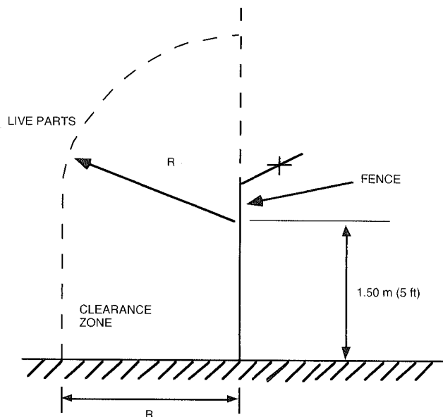
Figure 110-1—Safety clearance to electric supply station fences
