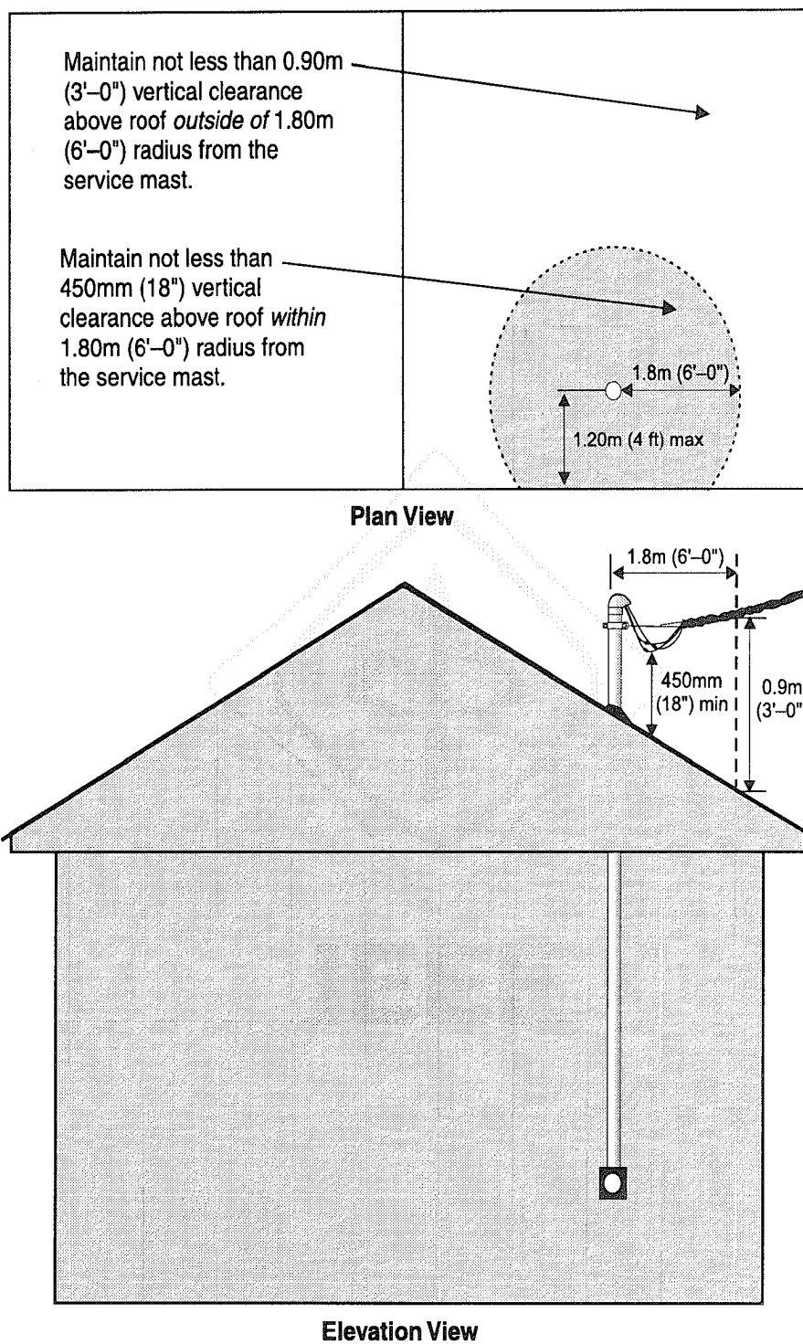
Fig 234-2 Clearances of Service Drop Terminating on Support Mast
