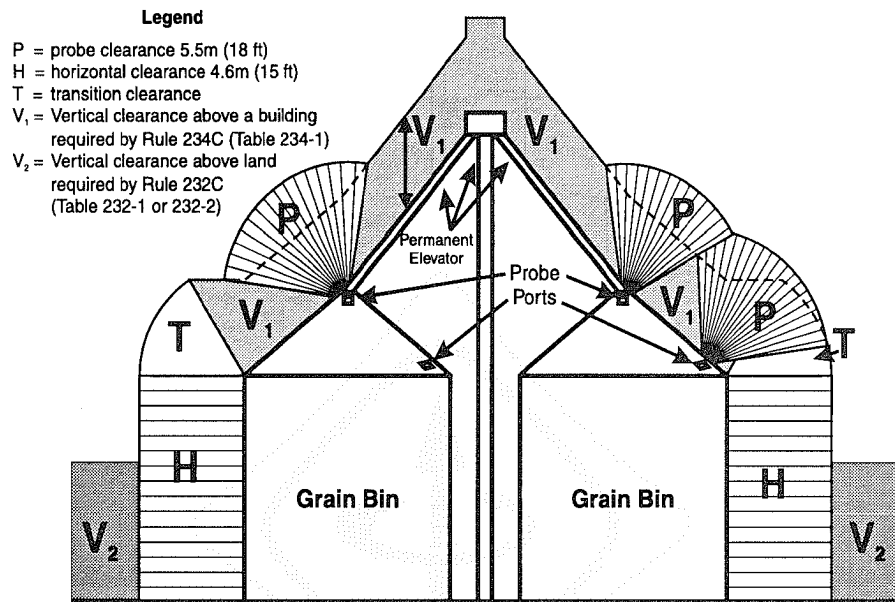
Fig 234-4(a) Clearance Envelope for Grain Bins Filled by Permanently Installed Augers, Conveyors, or Elevators
