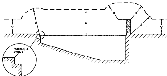
Fig 234-3 Swimming Pool Clearances
