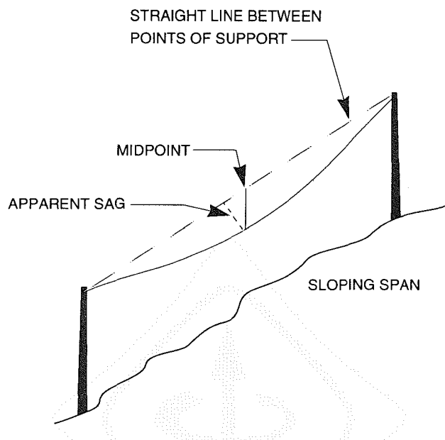
Figure D-1 Sag and Apparent Sag
