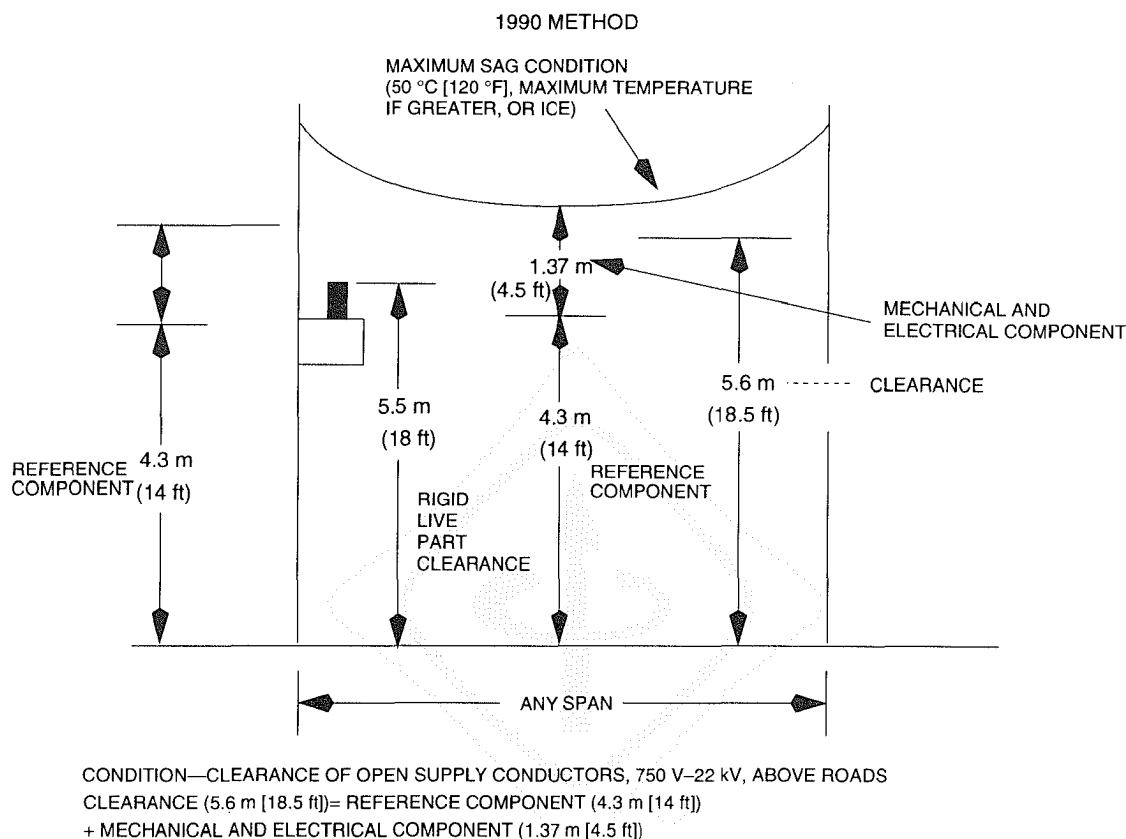
Fig A4 Clearance at Maximum Sag
