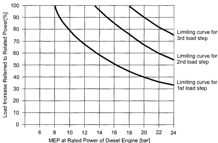
Figure 4/5 C.1—Limiting Curves for Loading 4-stroke Diesel Engines Step by Step from No-load to Rated Power as Function of the Brake Mean Effective Pressure
