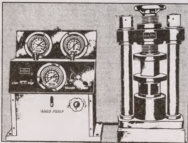
"ASEW" CONCRETE CUBE TESTING MACHINE
