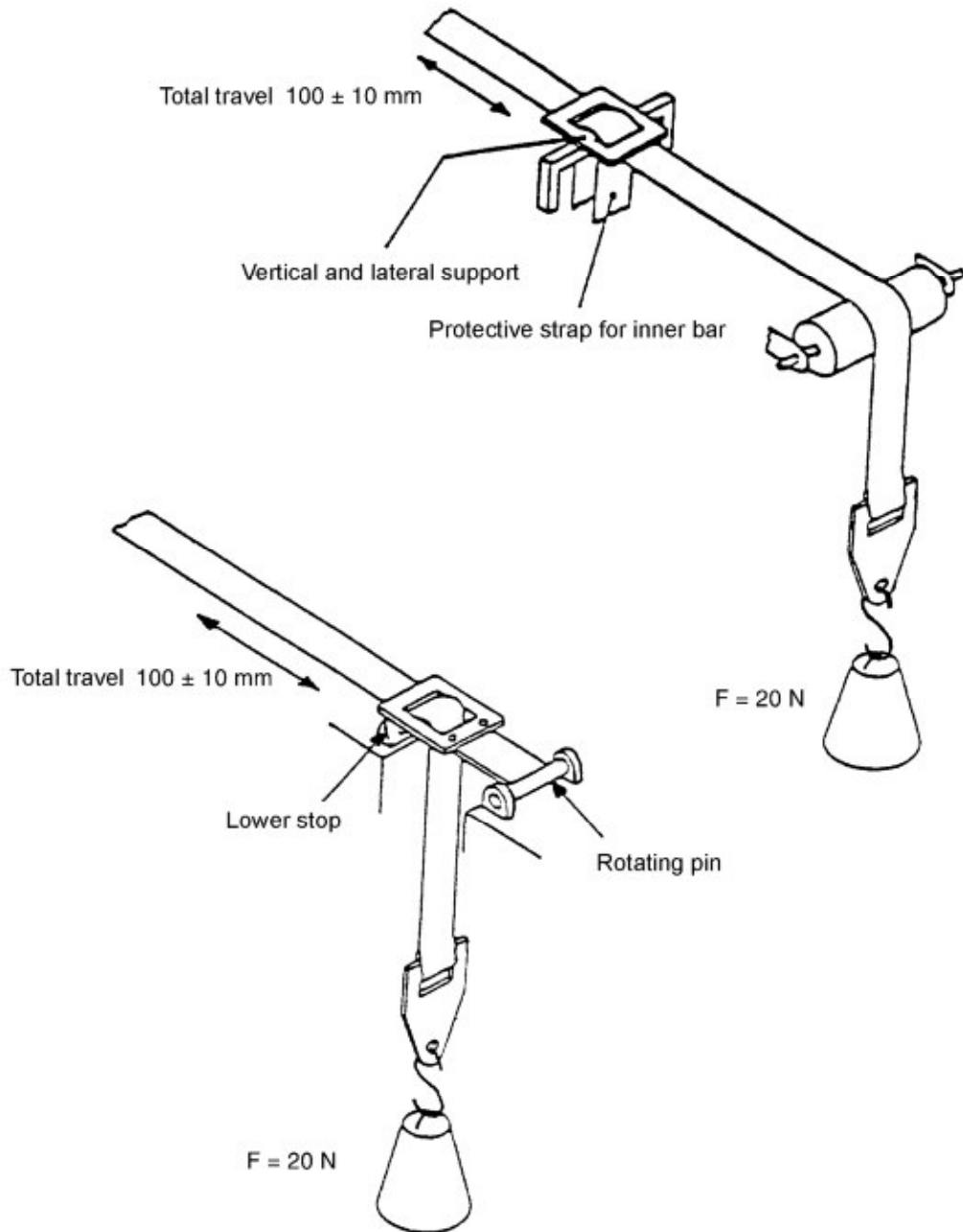
Figure 2 – Apparatus for Testing Abrasion of the Chin Strap
