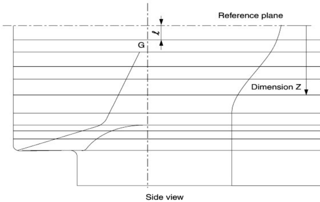
REFERENCE HEADFORMS (shape, dimensions below reference plane)
