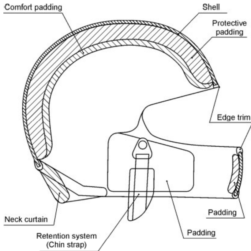
Figure 1 – Diagram of Protective Helmet
