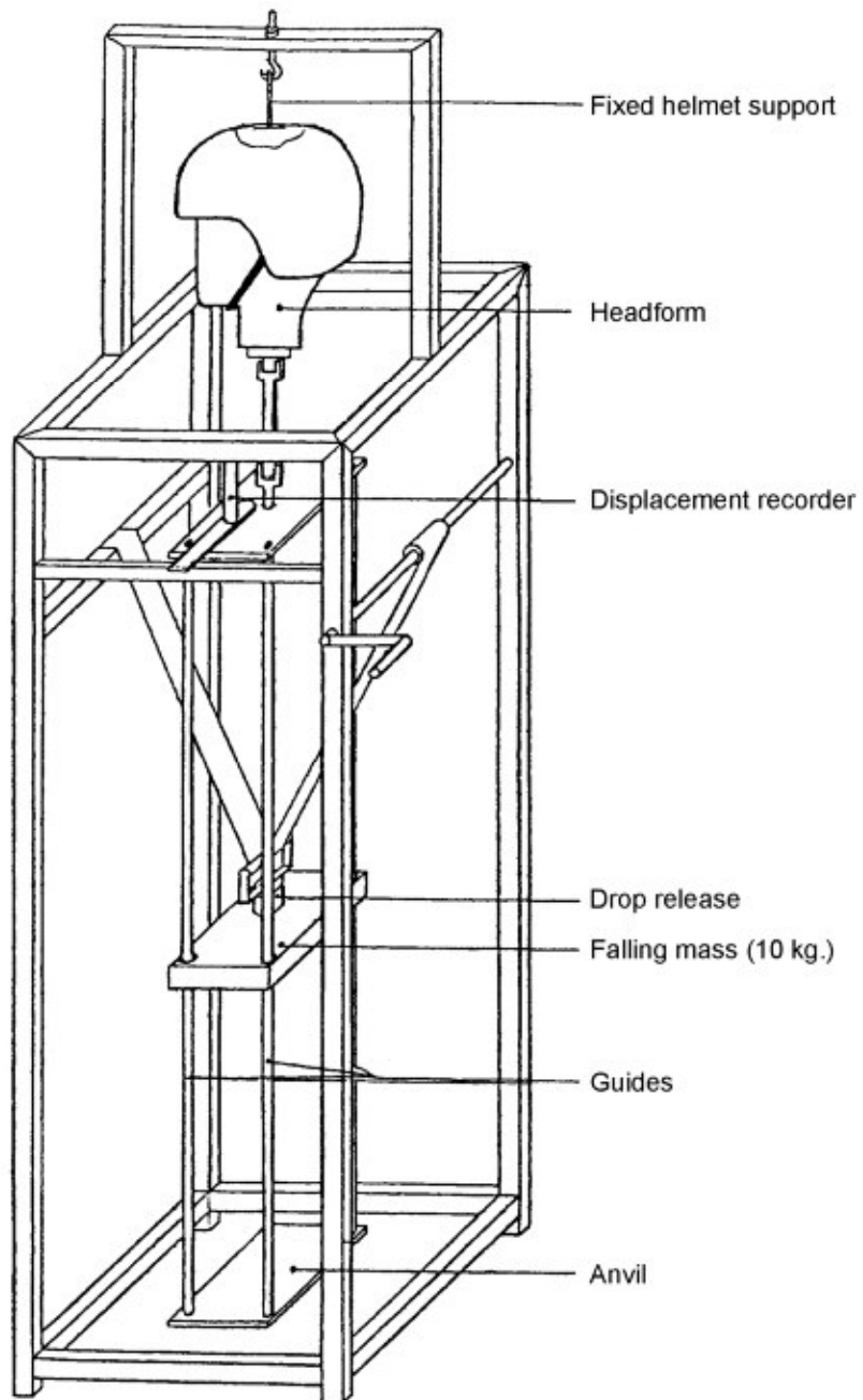
Figure 1 - Dynamic Test of Retention System
