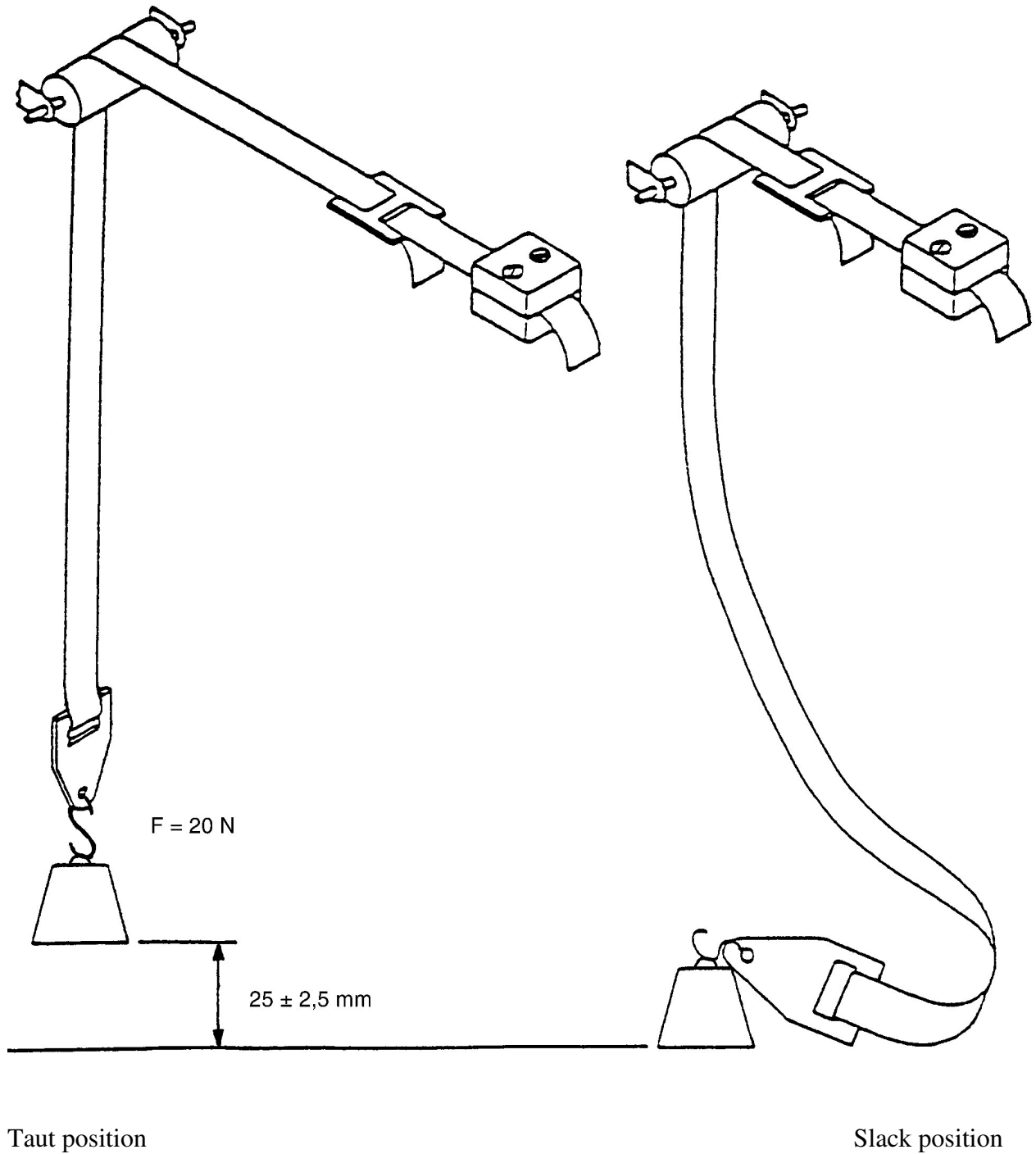
Figure 1 – APPARATUS FOR TESTING SLIPPAGE OF THE CHINSTRAP
