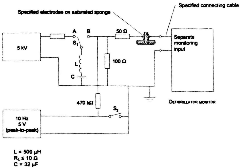
Figure 105 – Arrangement for recovery test after defibrillation (see 105.2)
