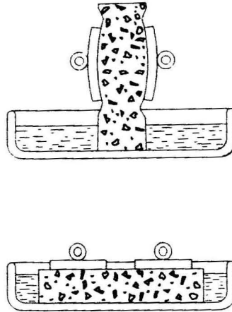
Figure 104 – Arrangement of monitoring electrodes on sponge (see 105.2)
