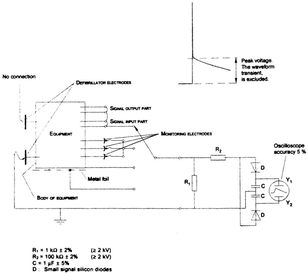
Figure 101 – Dynamic test for limitation of energy from different parts of the EQUIPMENT (see Item aa) of Clause 17)
