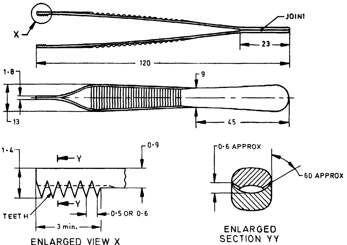
FIG. 1 TISSUE FORCEPS, ADSON-BROWN'S PATTERN
