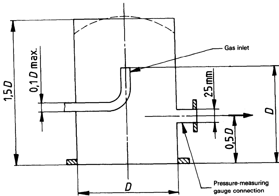
Figure 1 – Test dome
