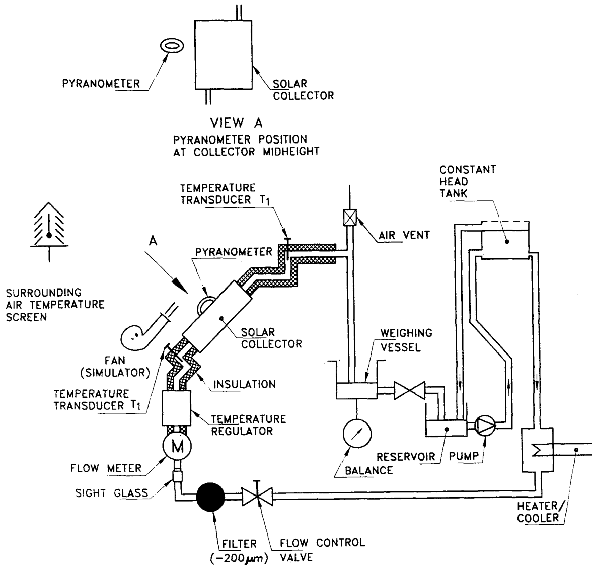
FIG. 5 AN EXAMPLE OF AN OPEN TEST LOOP
