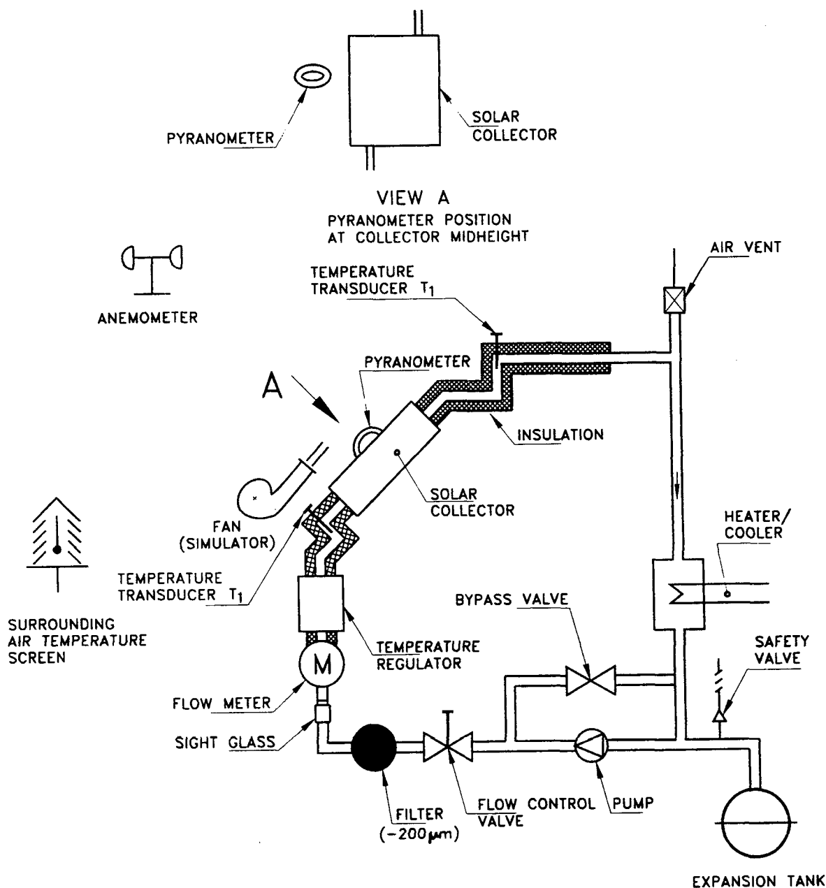
FIG. 6 AN EXAMPLE OF A CLOSED TEST LOOP
