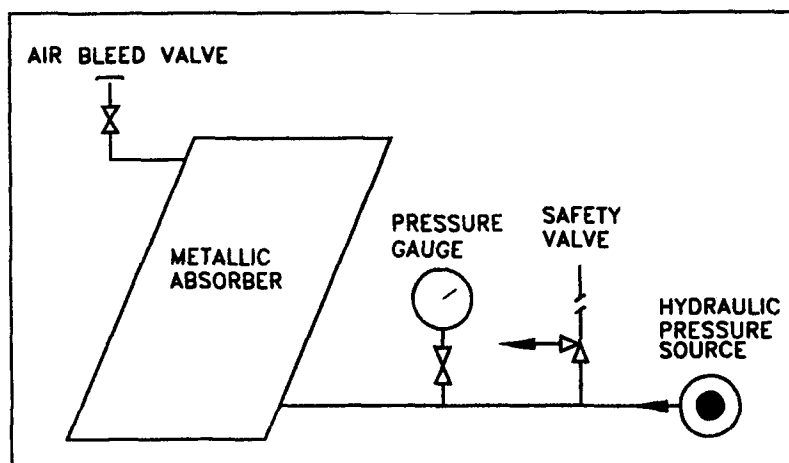
FIG. 1 TEST ARRANGEMENT FOR STATIC PRESSURE LEAKAGE TEST
