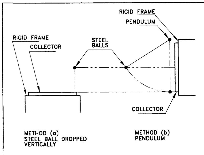
FIG. 4 IMPACT RESISTANCE TEST
