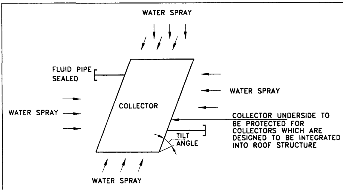
FIG. 3 RAIN PENETRATION TEST
