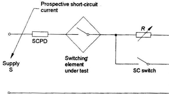
Figure H.3 – Short-circuit testing (see H.8.6.1)
