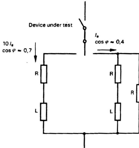
Figure C.1 – Normal circuit (see C.3.2.1)
