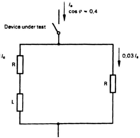
Figure C.2 – Simplified circuit (see C.3.2.1)
