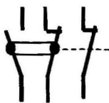
Figure L.1 – Example of representation of NO and NC contacts which are mechanically linked and NC non-linked contact
