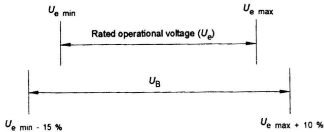
Figure H.1 – Relationship between U_e and U_B
