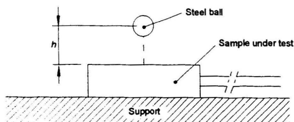
Figure F.2 – Test apparatus
