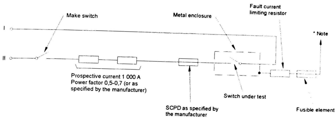
Figure 8 – Test circuit, conditional short-circuit current (see 8.3.4.2)
