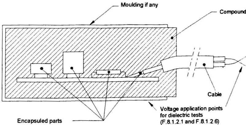
Figure F.1 – Insulation by encapsulation
