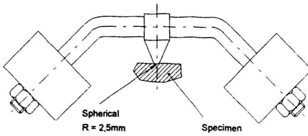
Figure 16 – Ball-pressure test apparatus
