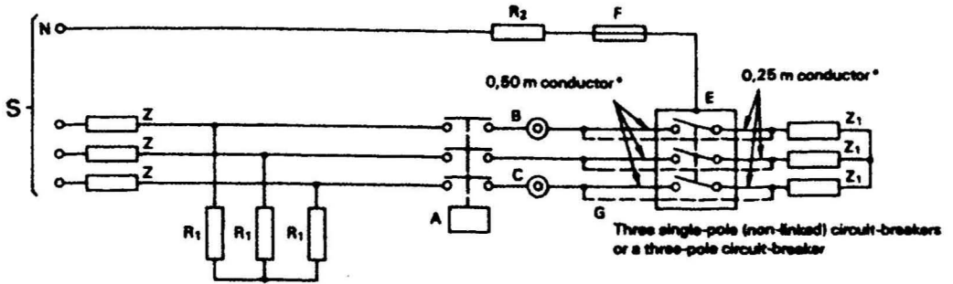
Figure 5 – Three-pole circuit-breaker (or three single-pole circuit-breakers)
