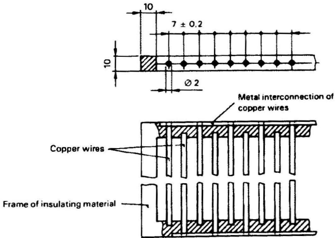
Figure H.2 – Grid circuit
