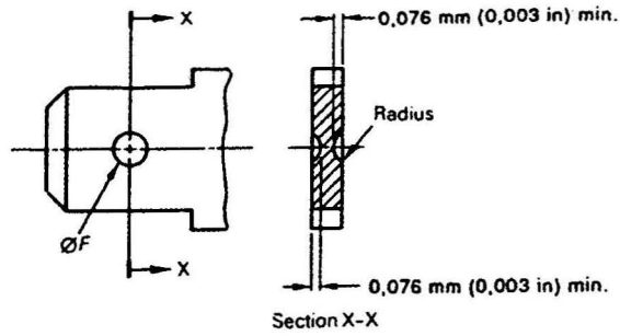
Figure K.3 – Dimensions of round dimple detents (see figure K.2)
