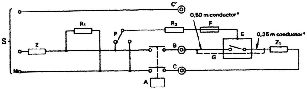
Figure 3 – Single pole circuit-breaker
