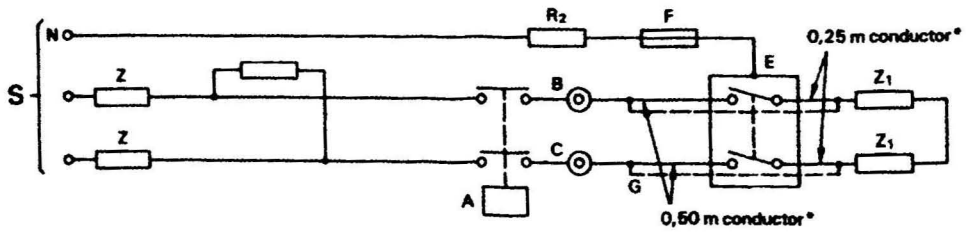
Figure 4b – Two-pole circuit-breaker with two protected poles
