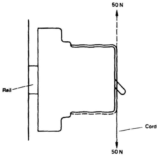
Figure 15 – Application of force for mechanical test on a rail-mounted circuit-breaker (9.13.2.3)
