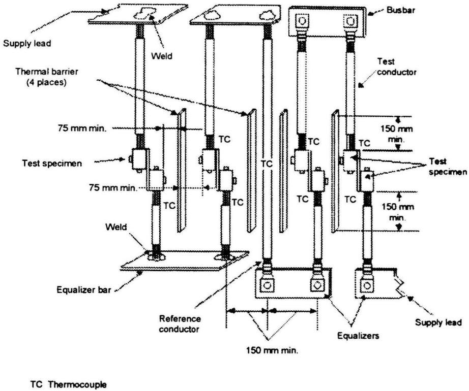
Figure L.1 – General arrangement for the test
