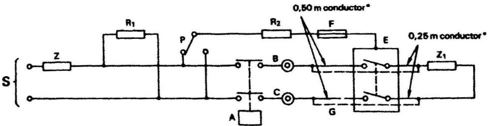
Figure 4a – Two-pole circuit-breaker with one protected pole
