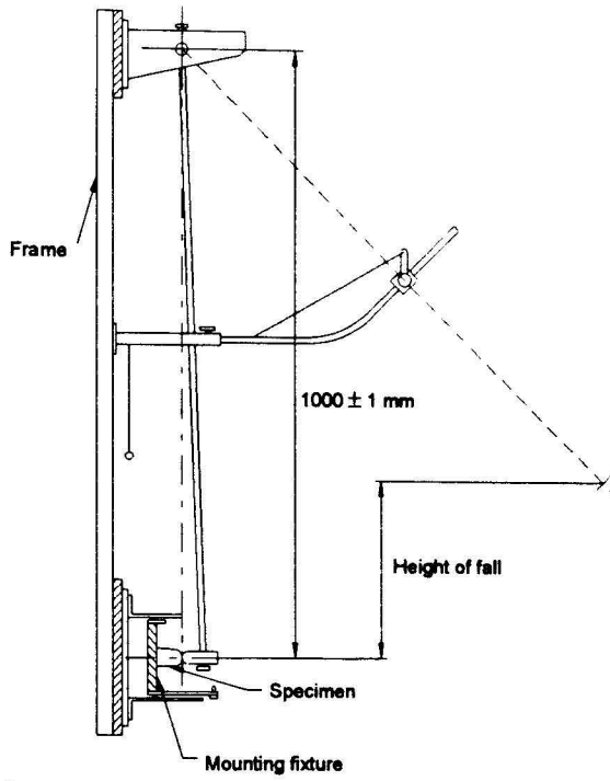
Figure 10 – Mechanical impact test apparatus (9.13.2)
