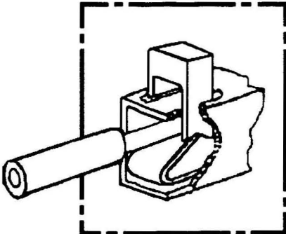
Figure J.2 – Examples of screwless-type terminals
