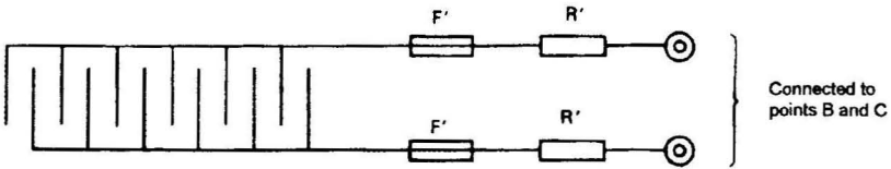
Figure H.3 – Grid circuit
