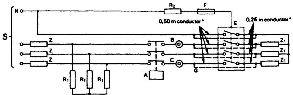
Figure 6 – Four-pole circuit-breaker
