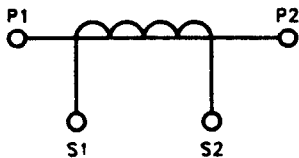
FIG. 1 SINGLE RATIO TRANSFORMER
