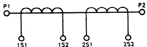
FIG. 4 TRANSFORMER WITH TWO SECONDARY WINDINGS
