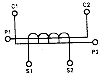
FIG. 3 TRANSFORMER WITH PRIMARY WINDING IN TWO SECTIONS INTENDED FOR CONNECTION EITHER IN SERIES OR PARALLEL
