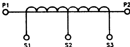
FIG. 2 TRANSFORMER WITH AN INTERMEDIATE TAPPING ON SECONDARY WINDING
