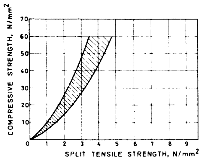
Fig. 33 Relationship Between Split Tensile Strength and Compressive Strength of Concrete
