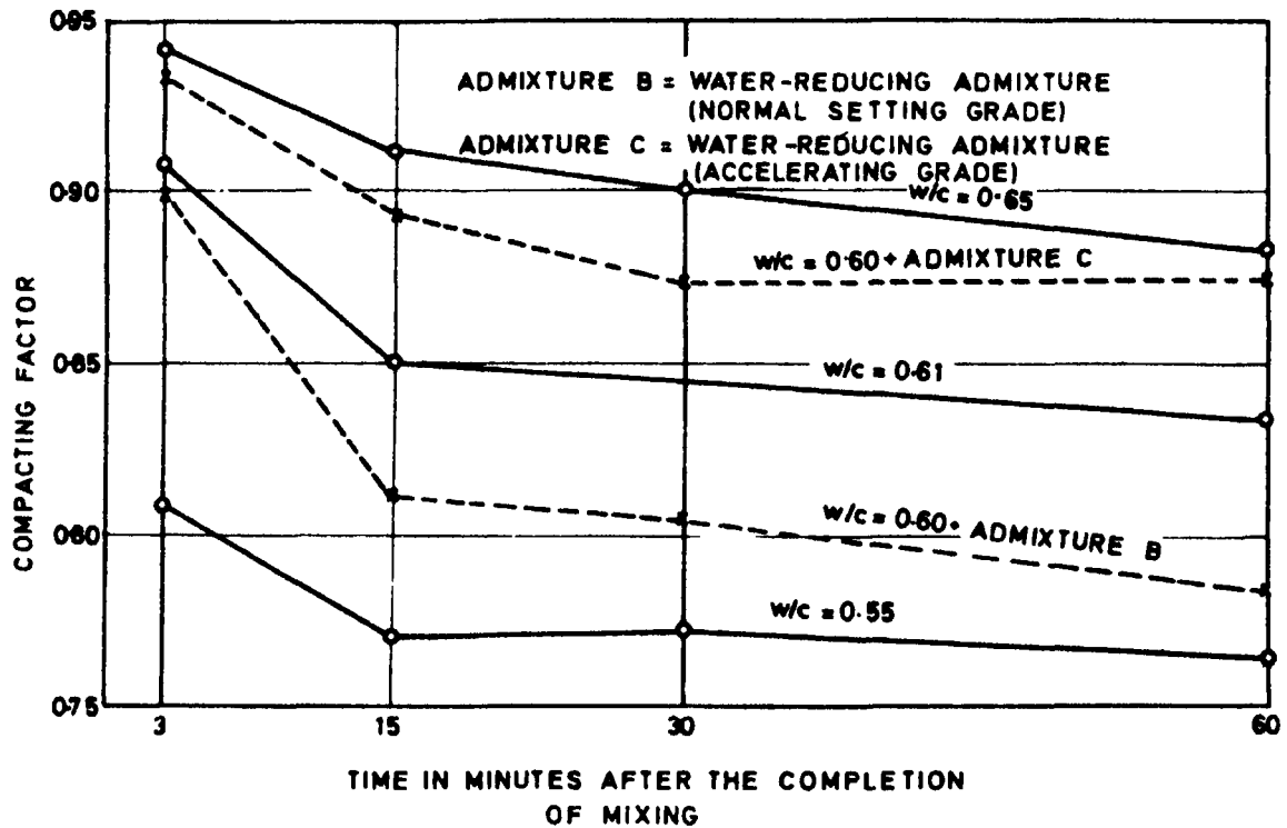
Fig. 21 Change in Compacting Factor with Time
