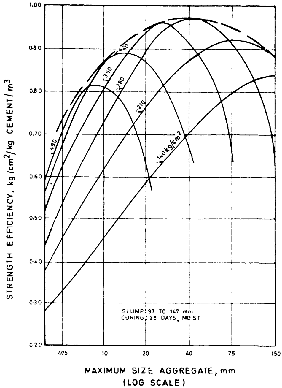
Fig. 41 Maximum Size Aggregate for Strength Efficiency Envelope
