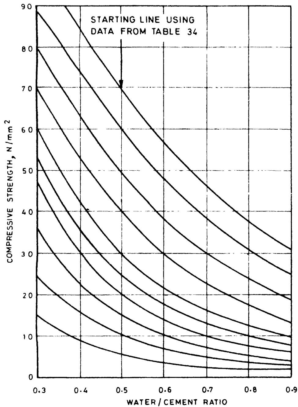
Fig. 43 Relationship Between Compressive Strength and Water-Cement Ratio
