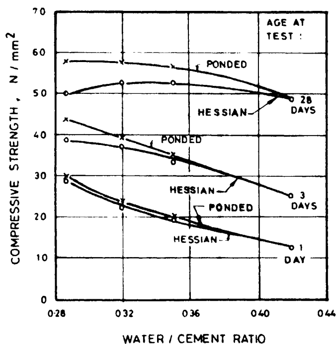
Fig. 28 Influence of Curing Conditions on Strength of Test Cylinders
