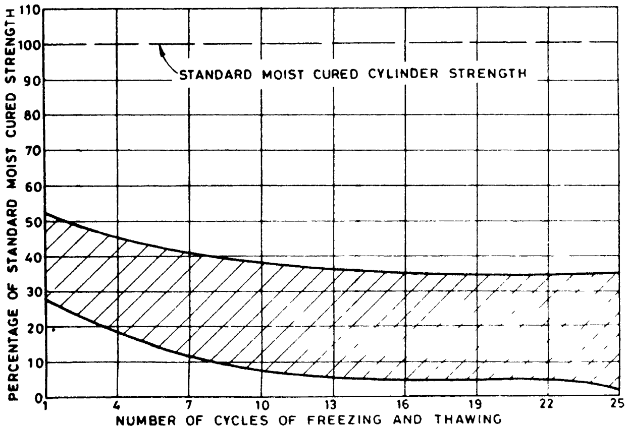
Fig. 52 Effect of Cycles of Freezing and Thawing of Fresh Concrete During Prehardening on Compressive Strength
