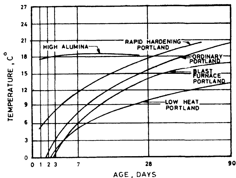
Fig. 4 Calculated Temperature Rise of Different Cements Under Adiabatic Conditions
