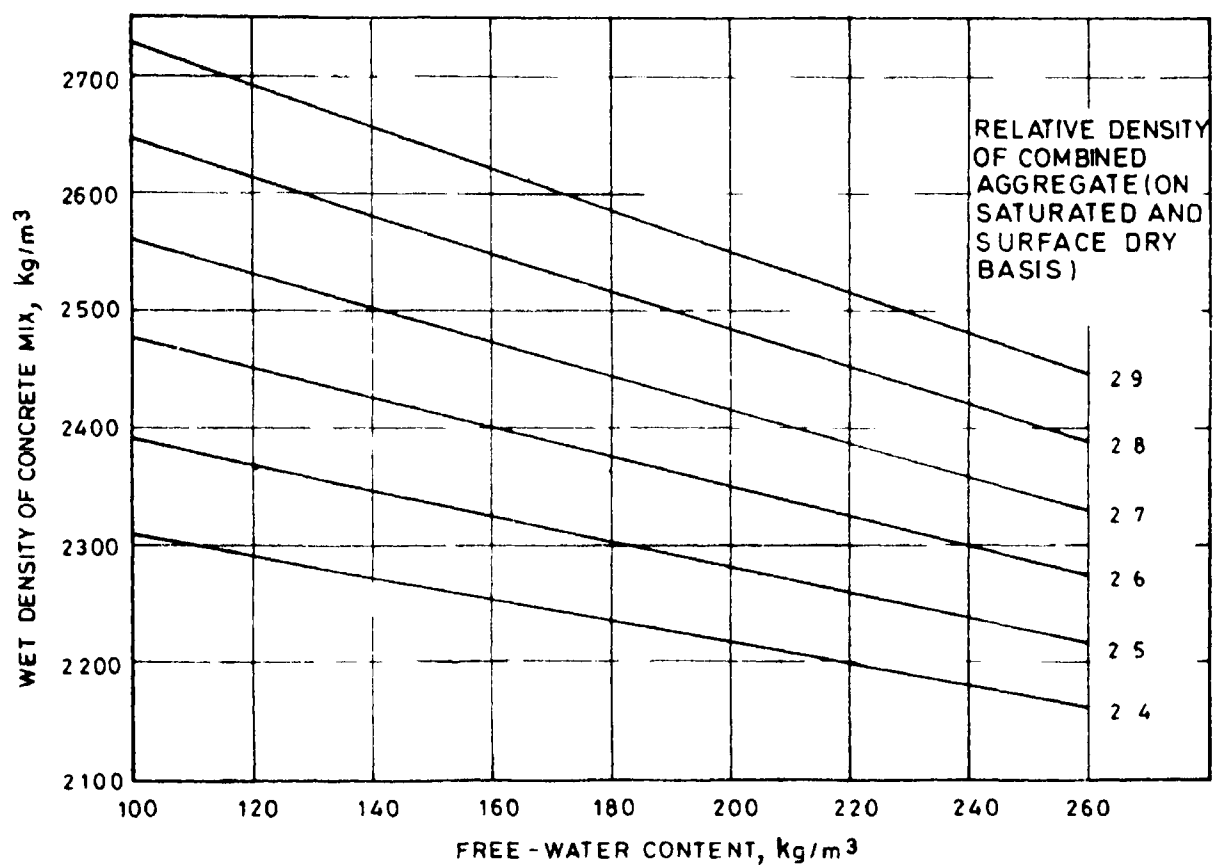
Fig. 44 Estimated Wet Density of Fully Compacted Concrete
