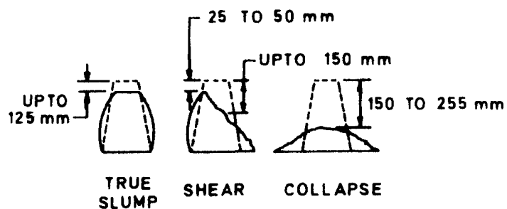
Fig. 18 Slump: True, Shear and Collapse
