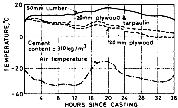
Fig. 54 Form Protection — 90 cm Concrete Cube, Thermocouple at Centre of Face (Next to Form)
