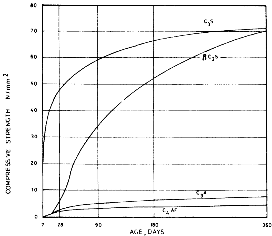
Fig. 2 Development of Strength of Pure Compounds
