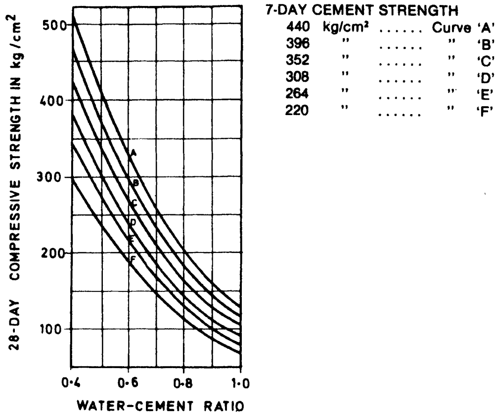
Fig. 25 Design Curve for Cement Concrete Mixes in Relation to 7-Day Compressive Strength of Cement
