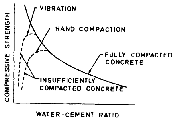
Fig. 26 Effect of Compaction on Compressive Strength of Concrete
