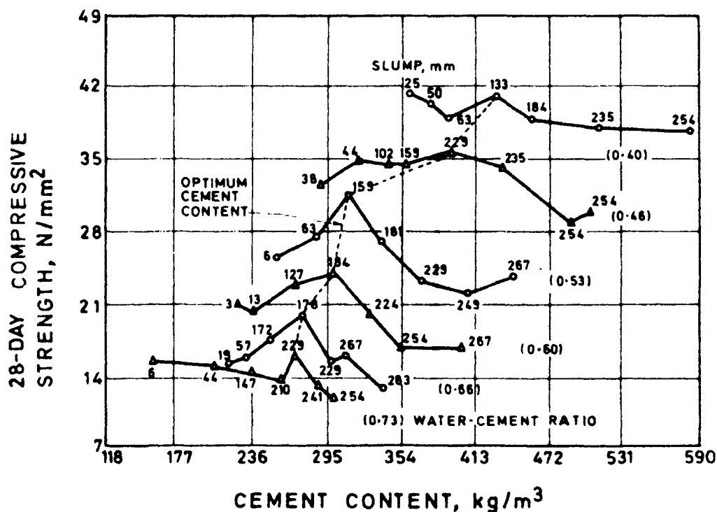
Fig. 24 Effect of Cement Content on the Compressive Strength of Concrete
