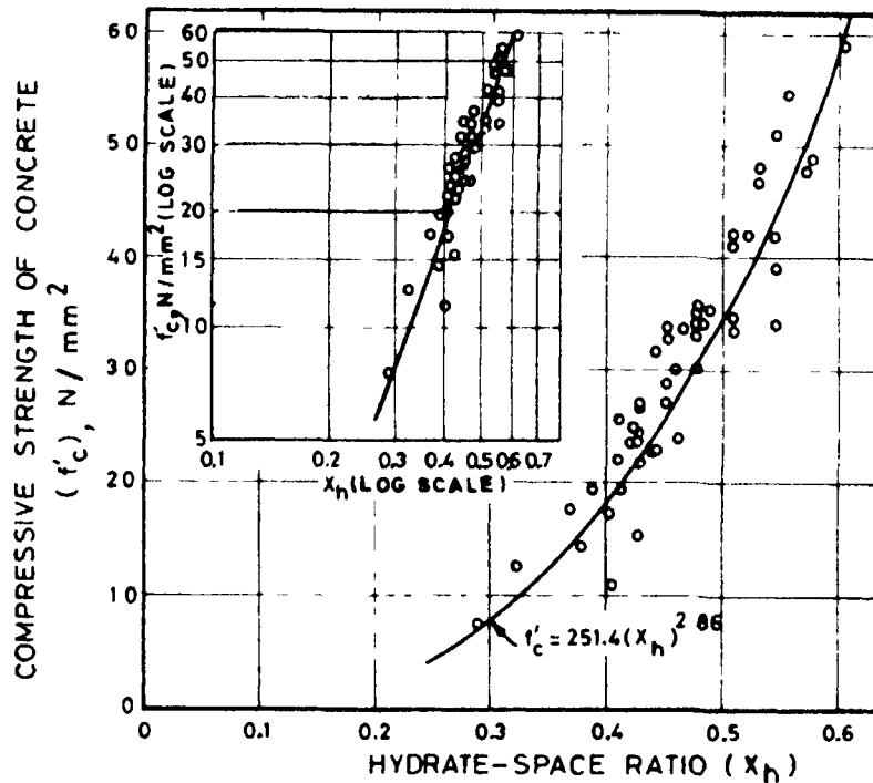
Fig. 6 Relationship Between Compressive Strength and Hydrate-Space Ratio
