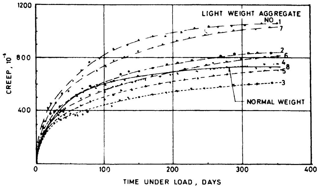
Fig. 13 Creep of Concrete of Nominal 210 kgf/cm 2 Strength Made with Different Lightweight Aggregates, Loaded at the Age of 7 Days to 42 kgf/cm 2
