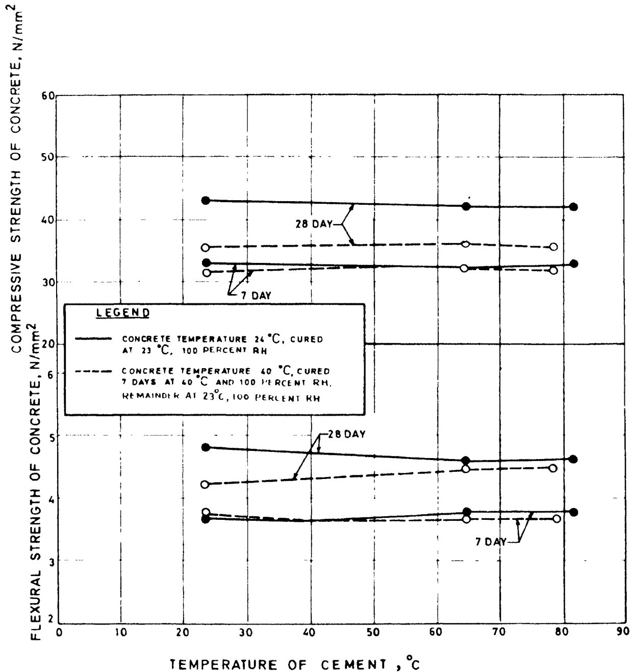
Fig. 50 Effect of Temperature of Cement on Concrete Strength
