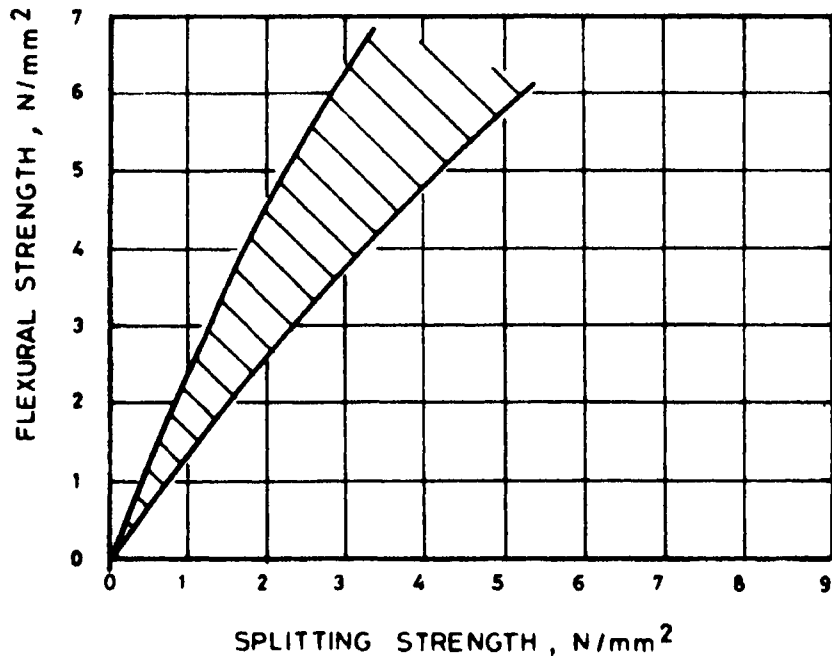
Fig. 35 Relationship Between Split Tensile Strength and Flexural Strength of Concrete
