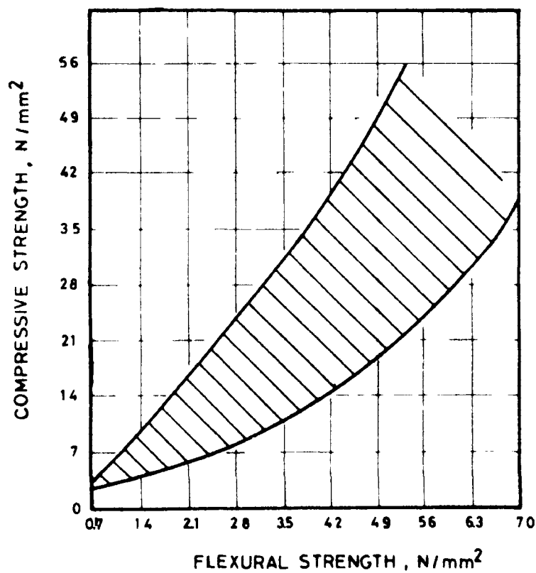
Fig. 34 Relationship Between Compressive and Flexural Strengths of Concrete
