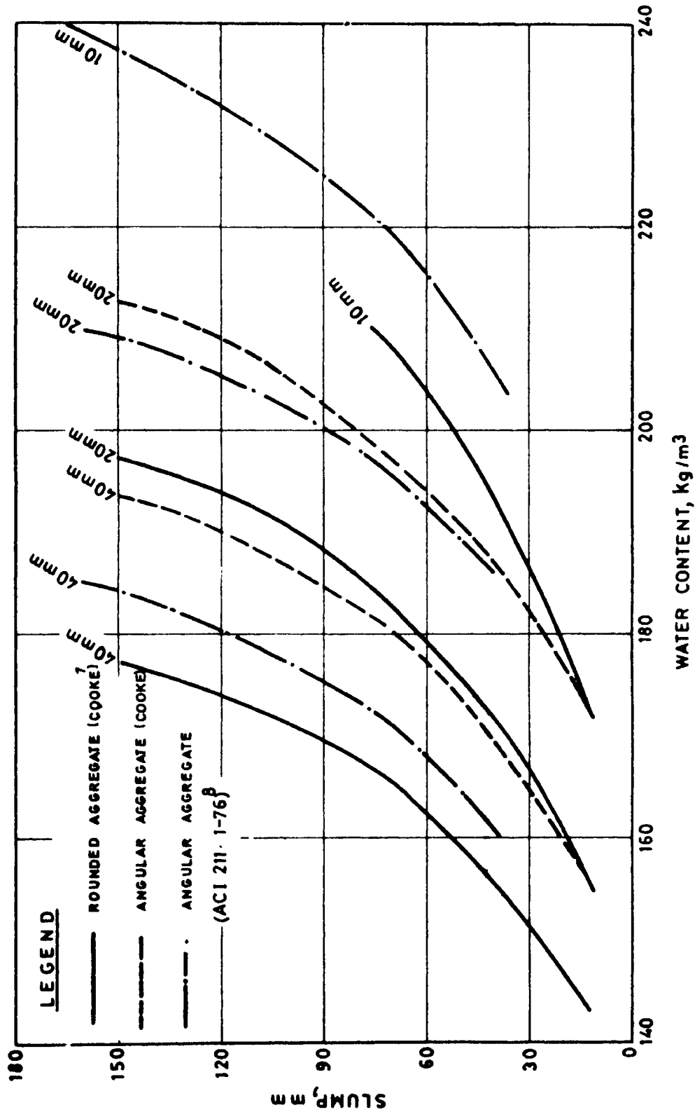
Fig. 20 Relationship Between Workability and Water Content of Concrete for Different Maximum Sizes of Aggregate
