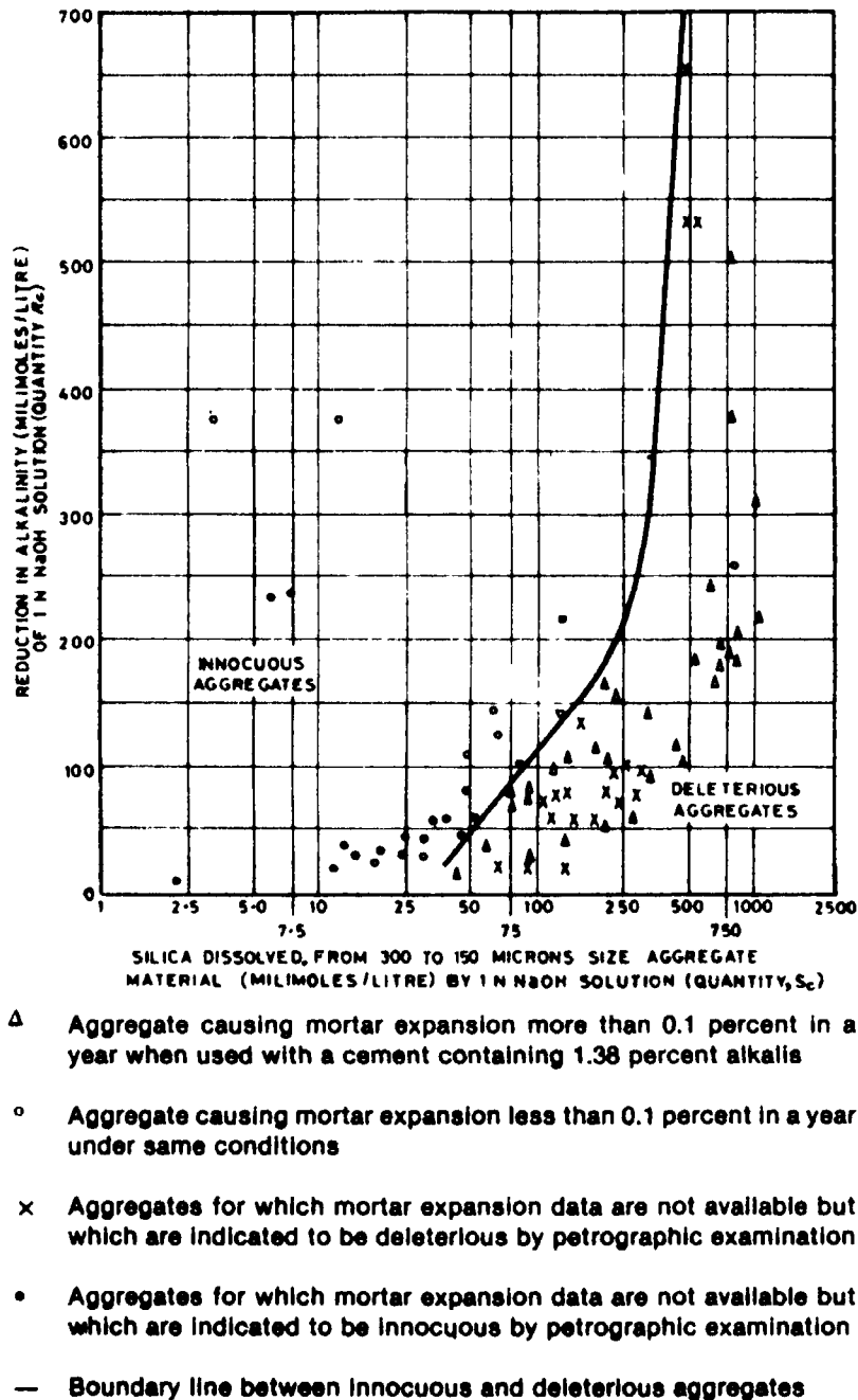
Fig. 12 Illustration of Division Between Innocuous and Deleterious Aggregates on Basis of Reduction in Alkalinity Test
