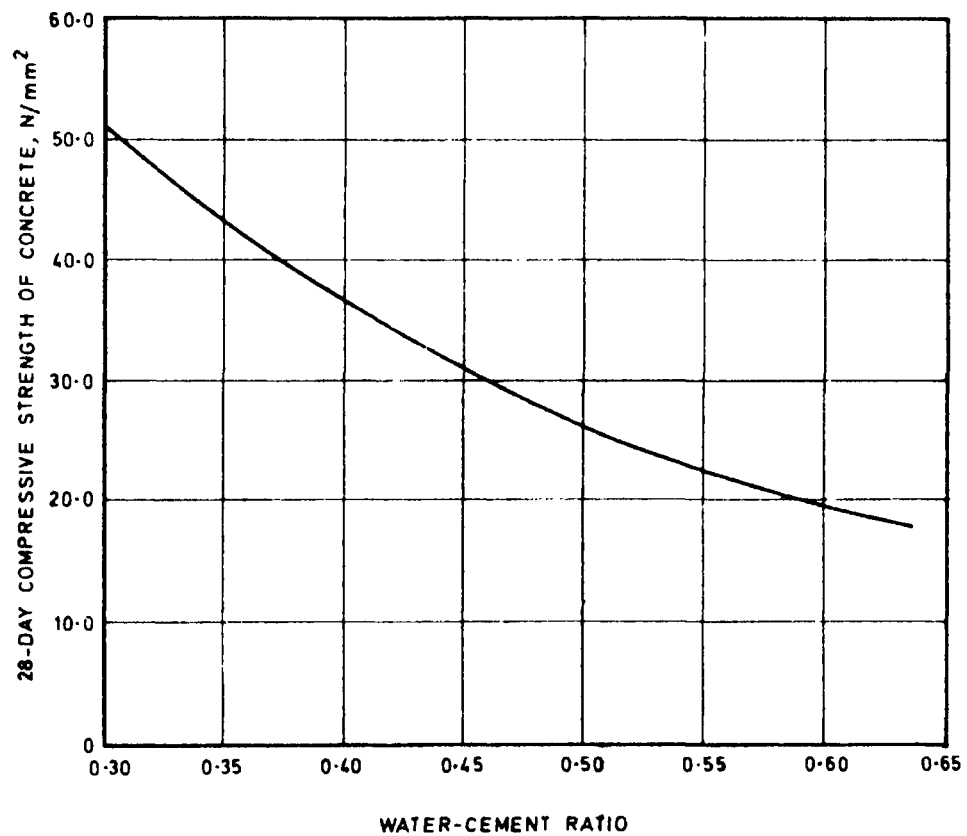
Fig. 46 Generalized Relationship Between Free Water-Cement Ratio and Compressive Strength of Concrete
