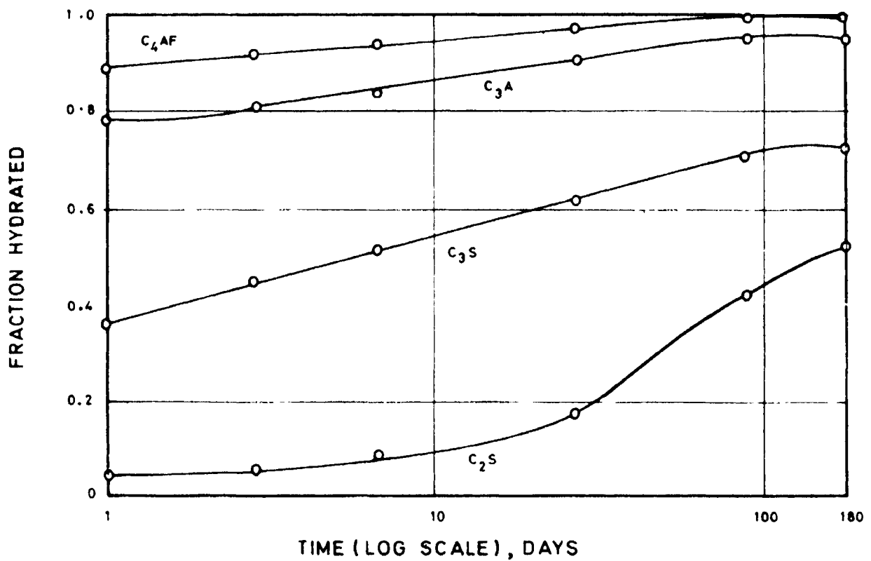
Fig. 1 Rate of Hydration of Pure Compounds
