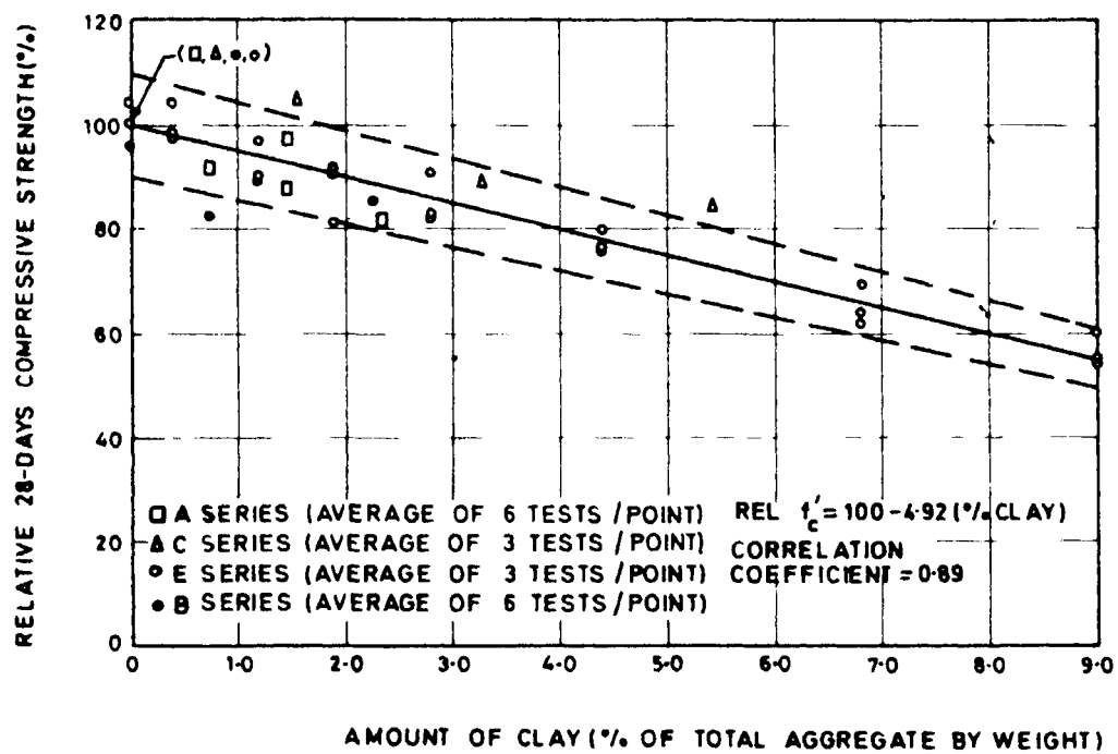
Fig. 11 Influence of Amount of Clay Fraction on 28-Day Compressive Strength
