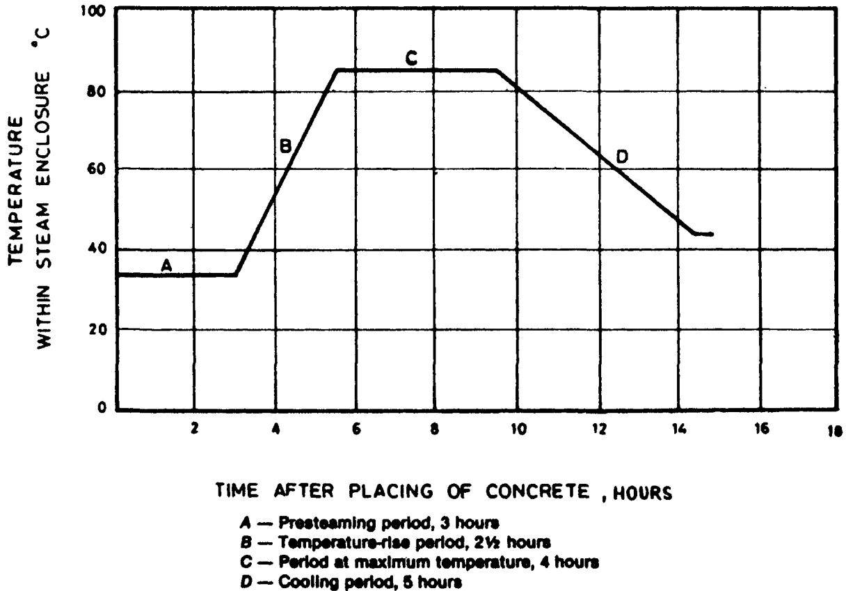
Fig. 30 Typical Steam Curing Cycle
