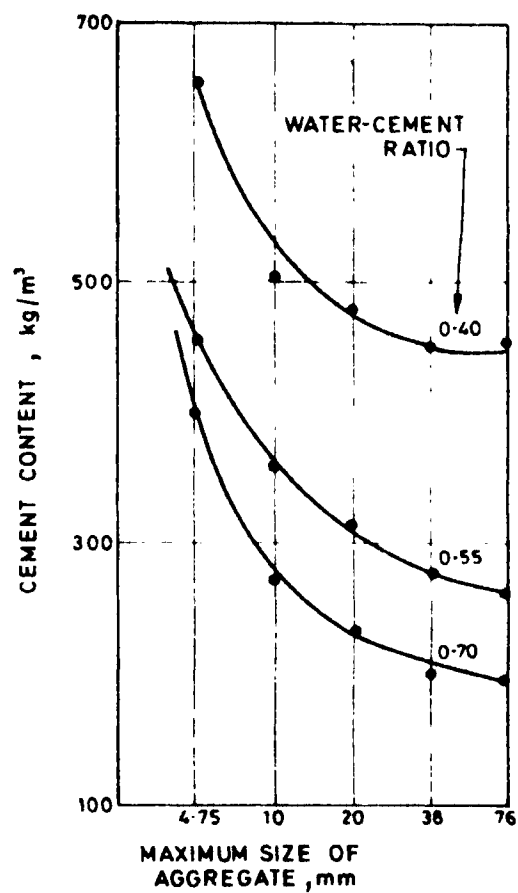
Fig. 40 Influence of Maximum Size of Aggregate on Cement Requirement of Concrete Mix
