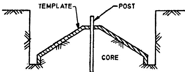
FIG. 9 CORE PROFILING FOR CONE
