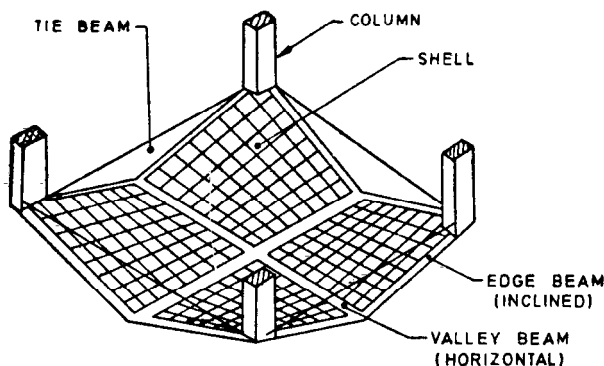
FIG. 8 INVERTED HIPPED HYPERBOLIC PARABOLOIDAL RAFT
