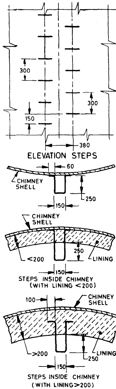
FIG. 5 STEPS FOR STEEL CHIMNEYS
