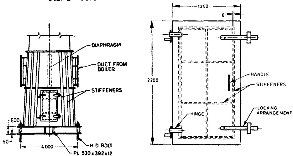
DETAIL OF DOOR
