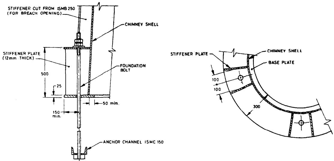
2A WELDED BASE
