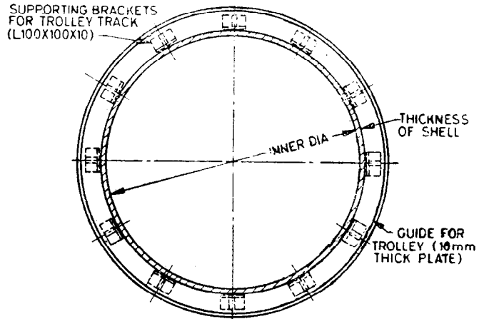
FIG. 7 TYPICAL DETAILS OF PAINTER'S TROLLEY ARRANGEMENT
