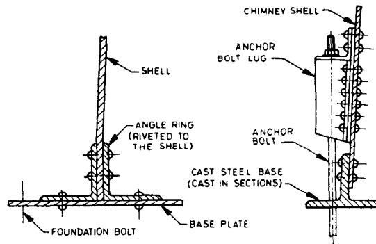
2B RIVETED BASE
