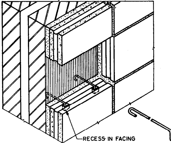
3 A TYPICAL FIXING DETAIL OF CRAMP
