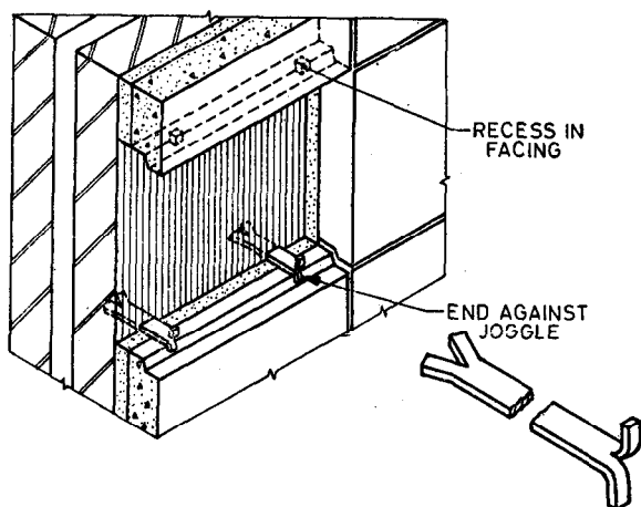
3D TYPICAL FIXING DETAIL OF CRAMP
