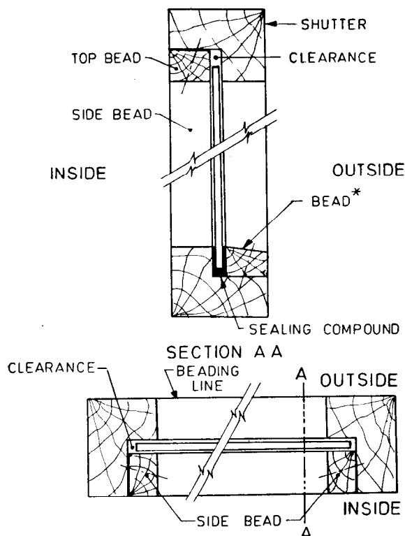
FIG. 3 INSIDE GLAZING
