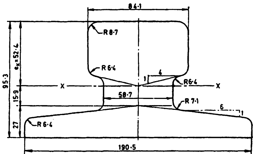
FIG. 7 74 kg/m CRANE RAIL SECTION
