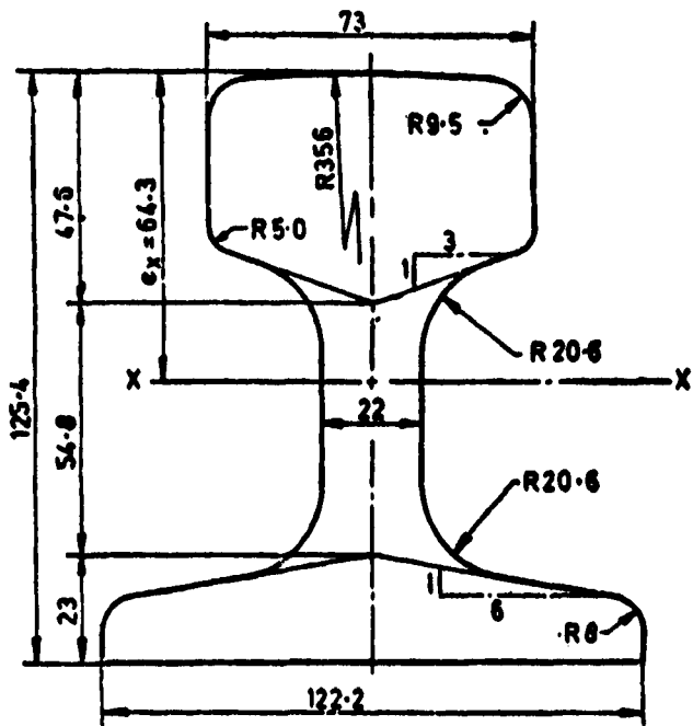
FIG. 5 52.2 kg/m CRANE RAIL SECTION
