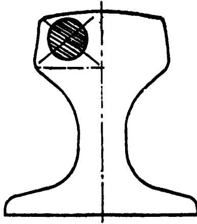
FIG. 1 LOCATION OF SAMPLE FOR CHEMICAL ANALYSIS AND TENSILE TESTING
