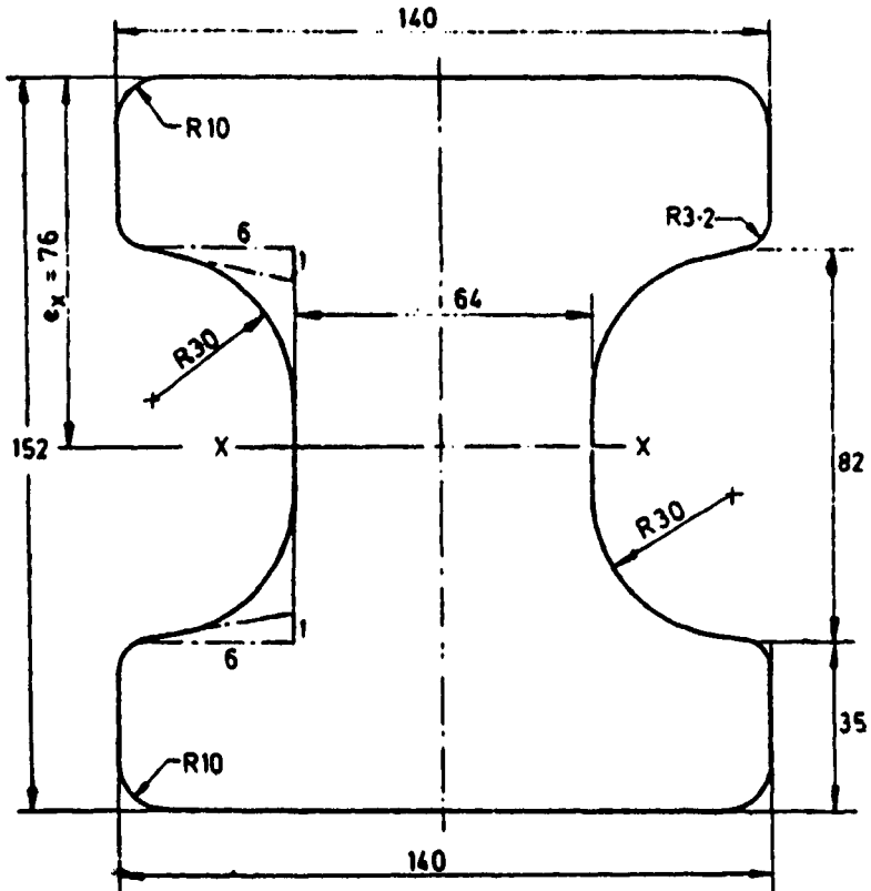
FIG. 8 125 kg/m CRANE RAIL SECTION
