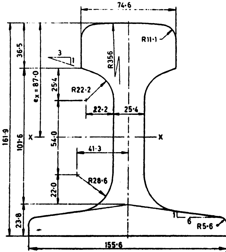
FIG. 6 67 kg/m CRANE RAIL SECTION
