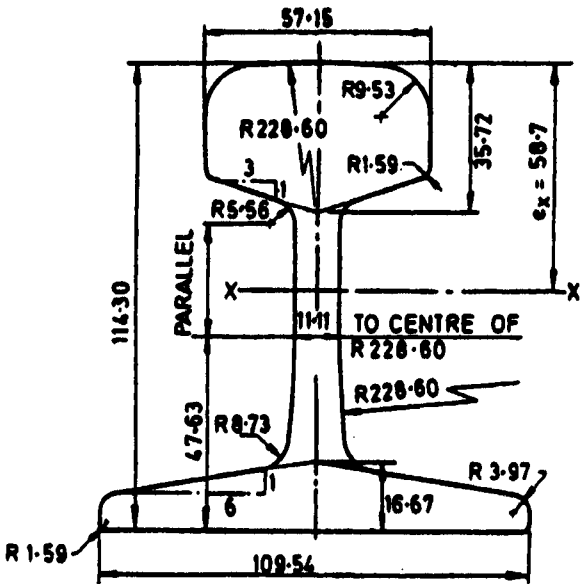
FIG. 2 30 kg/m CRANE RAIL SECTION
