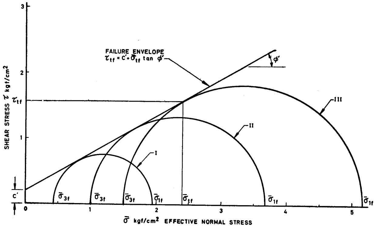
FIG. 6 STRESS CONDITIONS AT FAILURE IN TERMS OF EFFECTIVE STRESSES
