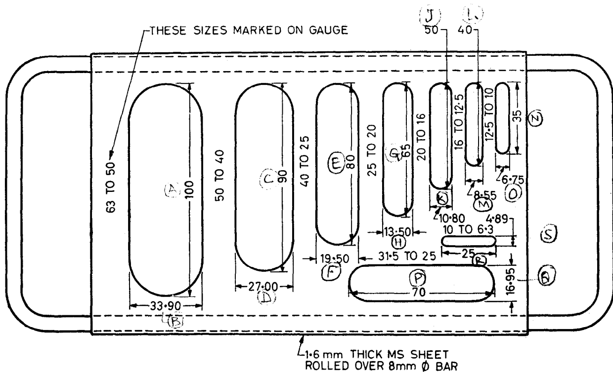
FIG. 2 THICKNESS GAUGE
