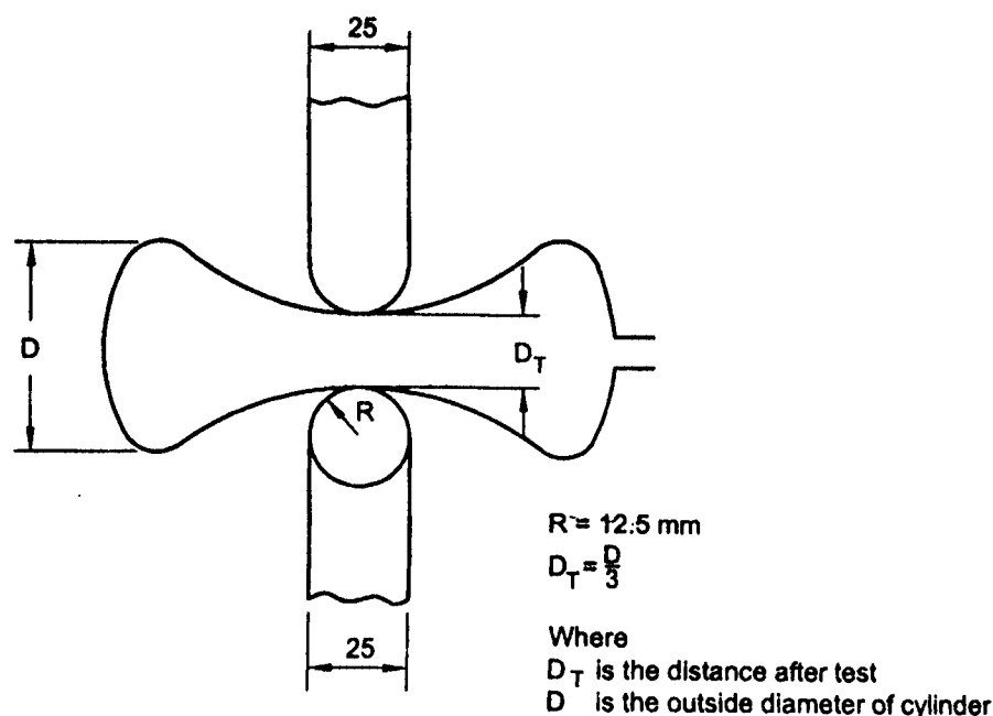
FIG. 4 CRUSHING TEST
