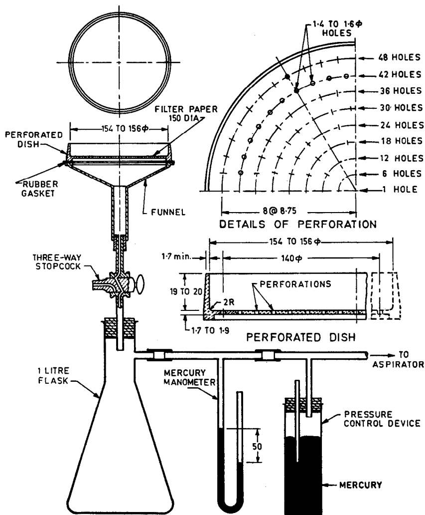
FIG. 1 APPARATUS ASSEMBLY FOR WATER RETENTION TEST
